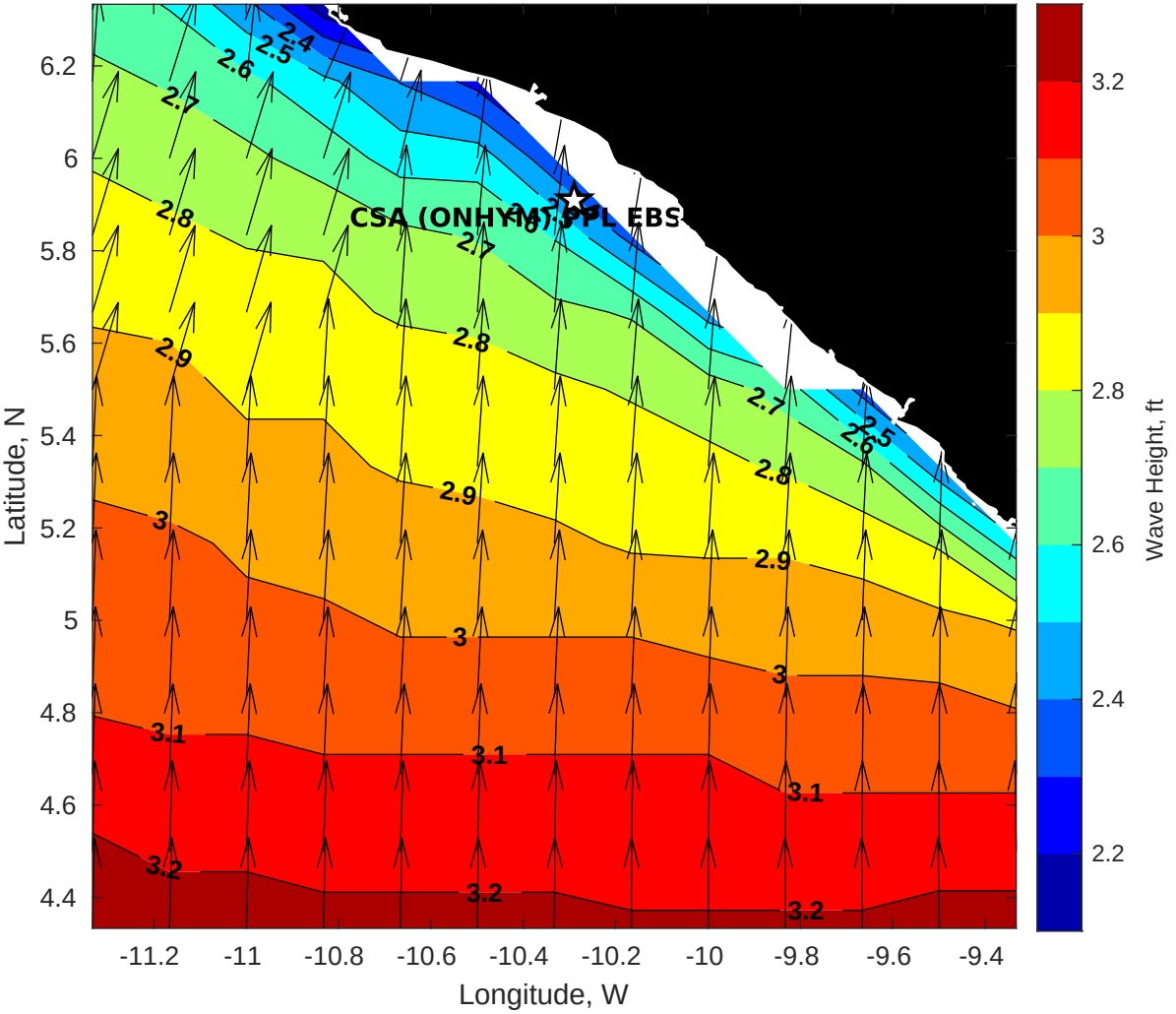
GFS Wave Height (ft) for CSA (ONHYM) PPL EBS - Liberia at 04-Dec-2025 09:00:00
