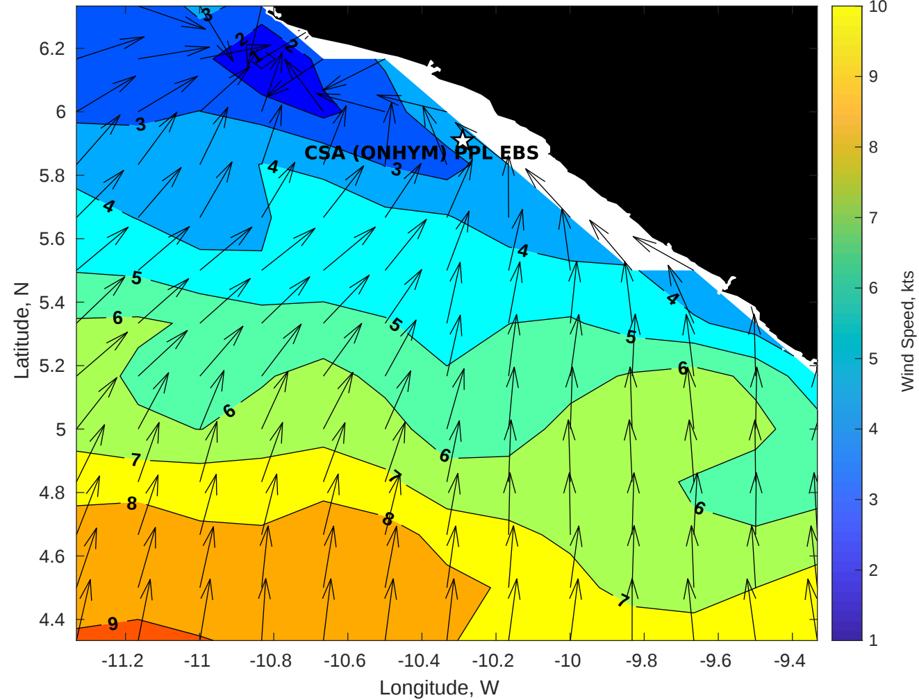
GFS Winds (kts) for CSA (ONHYM) PPL EBS - Liberia at 04-Dec-2025 09:00:00
