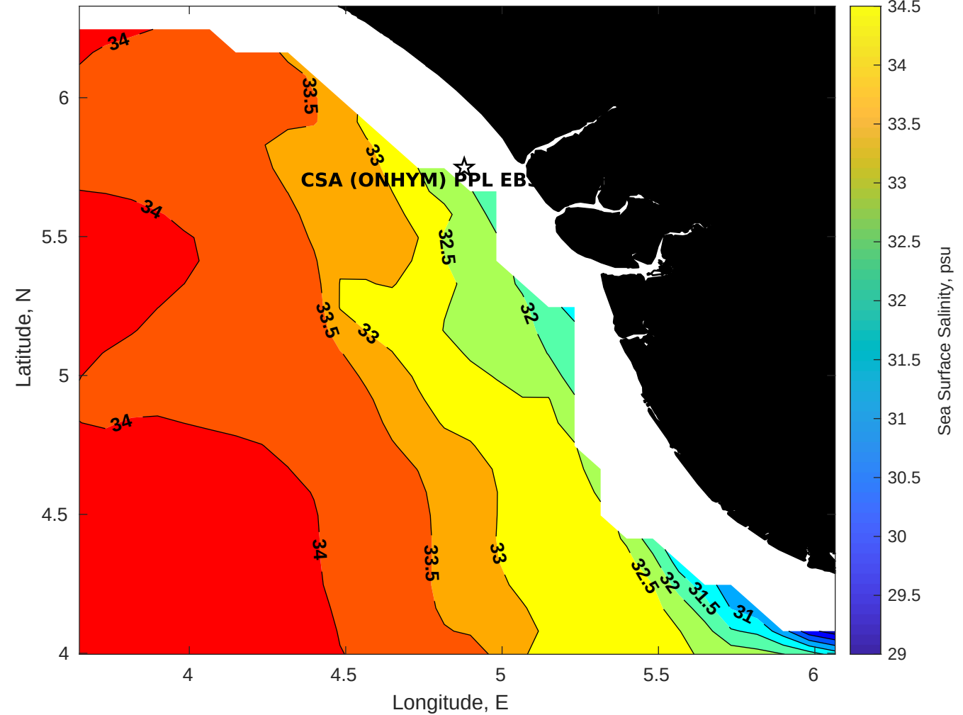
Surface Salinity for CSA (ONHYM) PPL EBS - Nigeria at 03-Dec-2025 00:00:00
