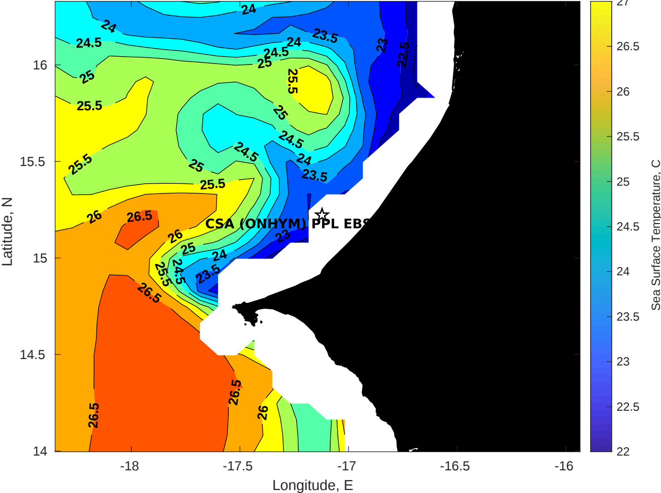
SST for CSA (ONHYM) PPL EBS - Senegal at 03-Dec-2025 00:00:00
