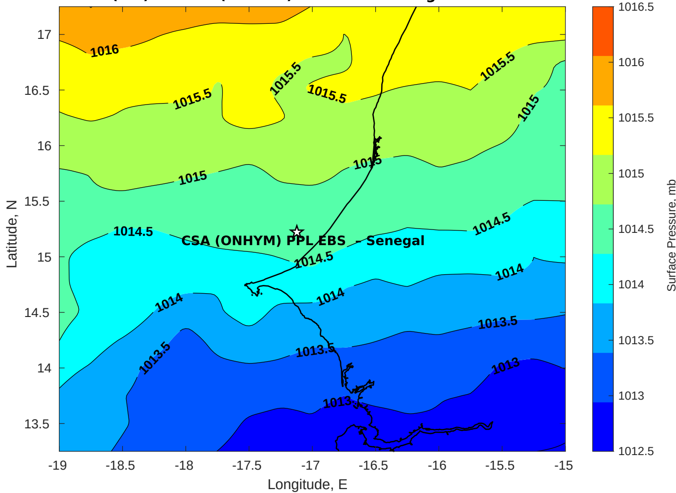
Surface Pressure (mb) for CSA (ONHYM) PPL EBS - Senegal at 06-Dec-2025 00:00:00
