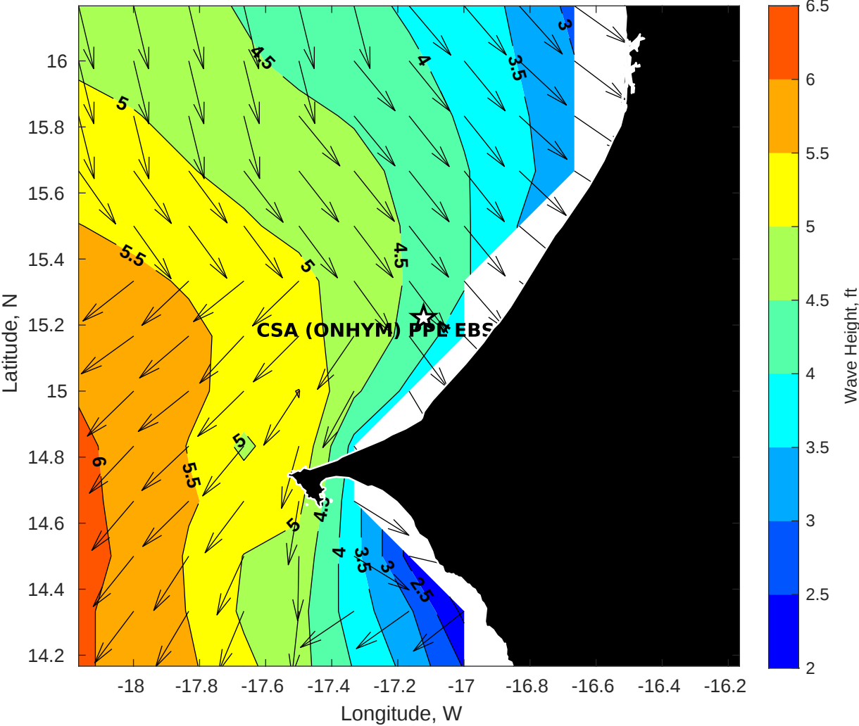
GFS Wave Height (ft) for CSA (ONHYM) PPL EBS - Senegal at 04-Dec-2025 09:00:00
