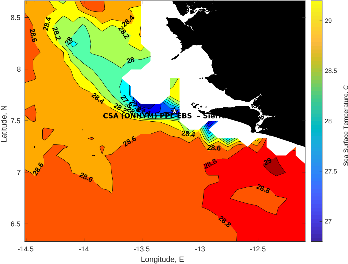
SST for CSA (ONHYM) PPL EBS - Sierra Leone at 03-Dec-2025 00:00:00
