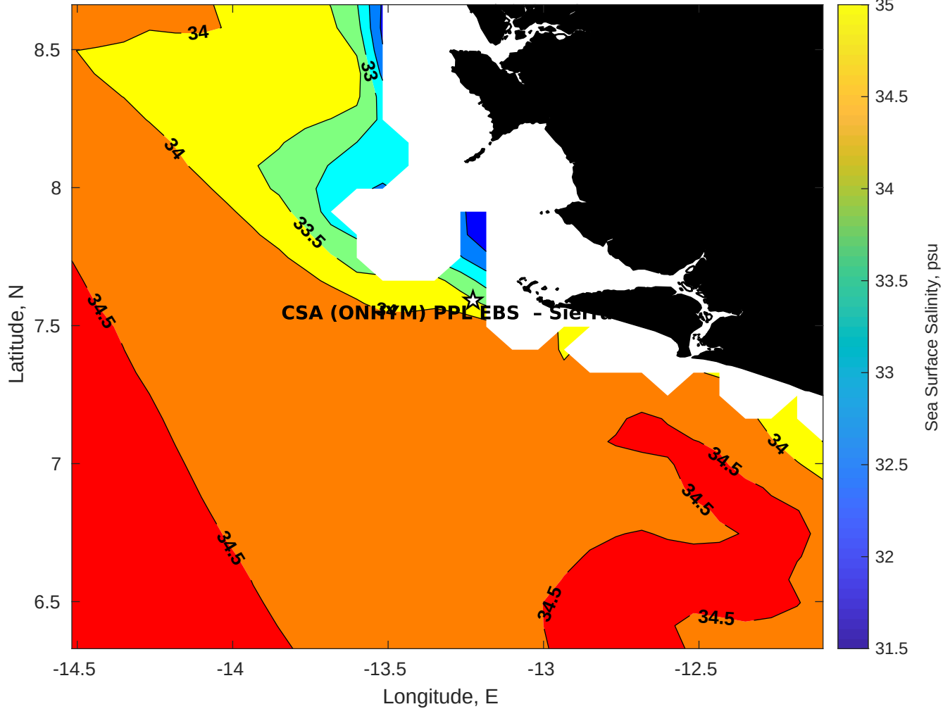
Surface Salinity for CSA (ONHYM) PPL EBS - Sierra Leone at 03-Dec-2025 00:00:00
