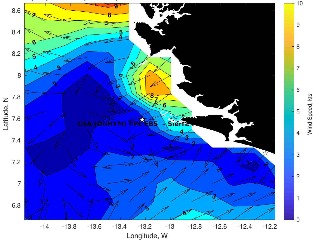
GFS Winds (kts) for CSA (ONHYM) PPL EBS - Sierra Leone at 04-Dec-2025 09:00:00
