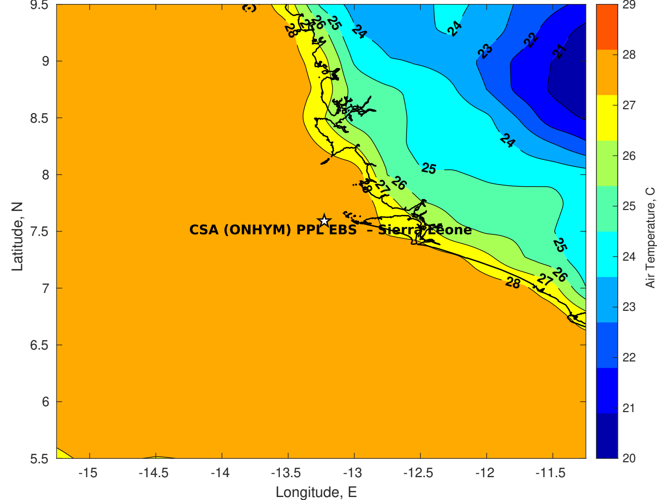
Air Temperature (C) for CSA (ONHYM) PPL EBS - Sierra Leone at 04-Dec-2025
