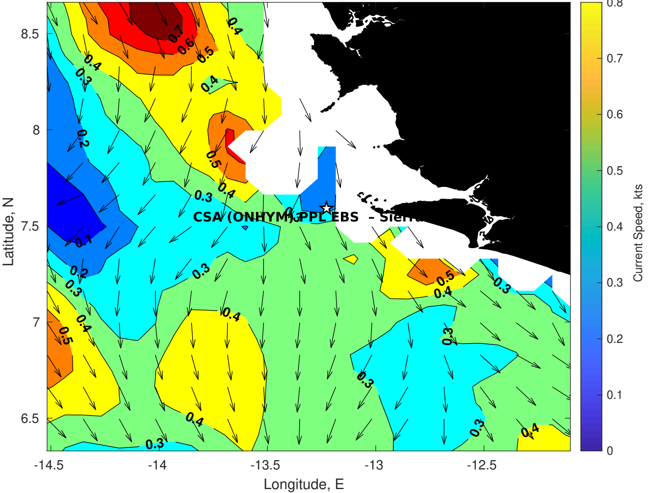
Surface Currents for CSA (ONHYM) PPL EBS - Sierra Leone at 03-Dec-2025 00:00:00
