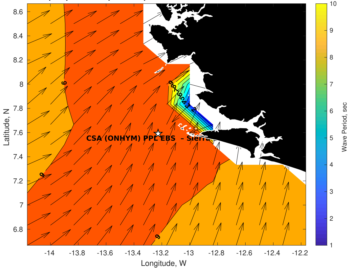
GFS Wave Period (sec) for CSA (ONHYM) PPL EBS - Sierra Leone at 04-Dec-2025 09:00:00
