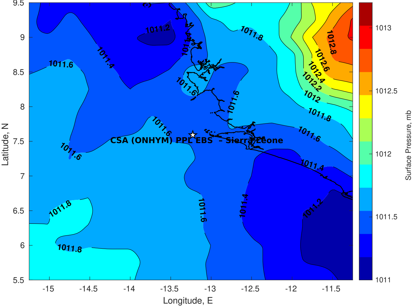
Surface Pressure (mb) for CSA (ONHYM) PPL EBS - Sierra Leone at 05-Dec-2025 00:00:00
