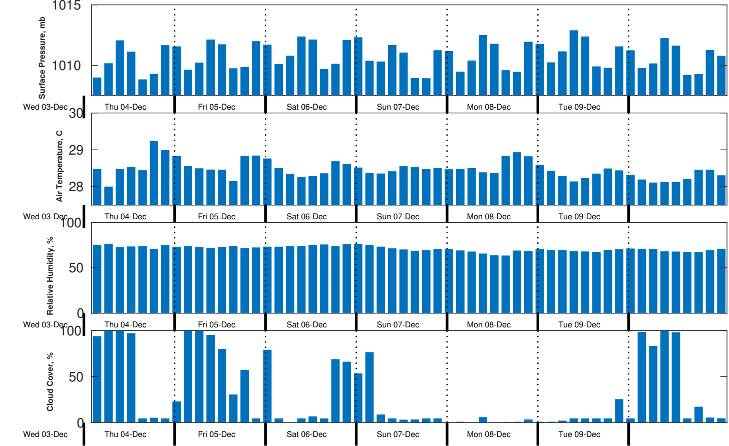
Met Forecast for CSA (ONHYM) PPL EBS - Sierra Leone from 04-Dec-2025 00:00:00 to 11-Dec-2025 00:00:00
