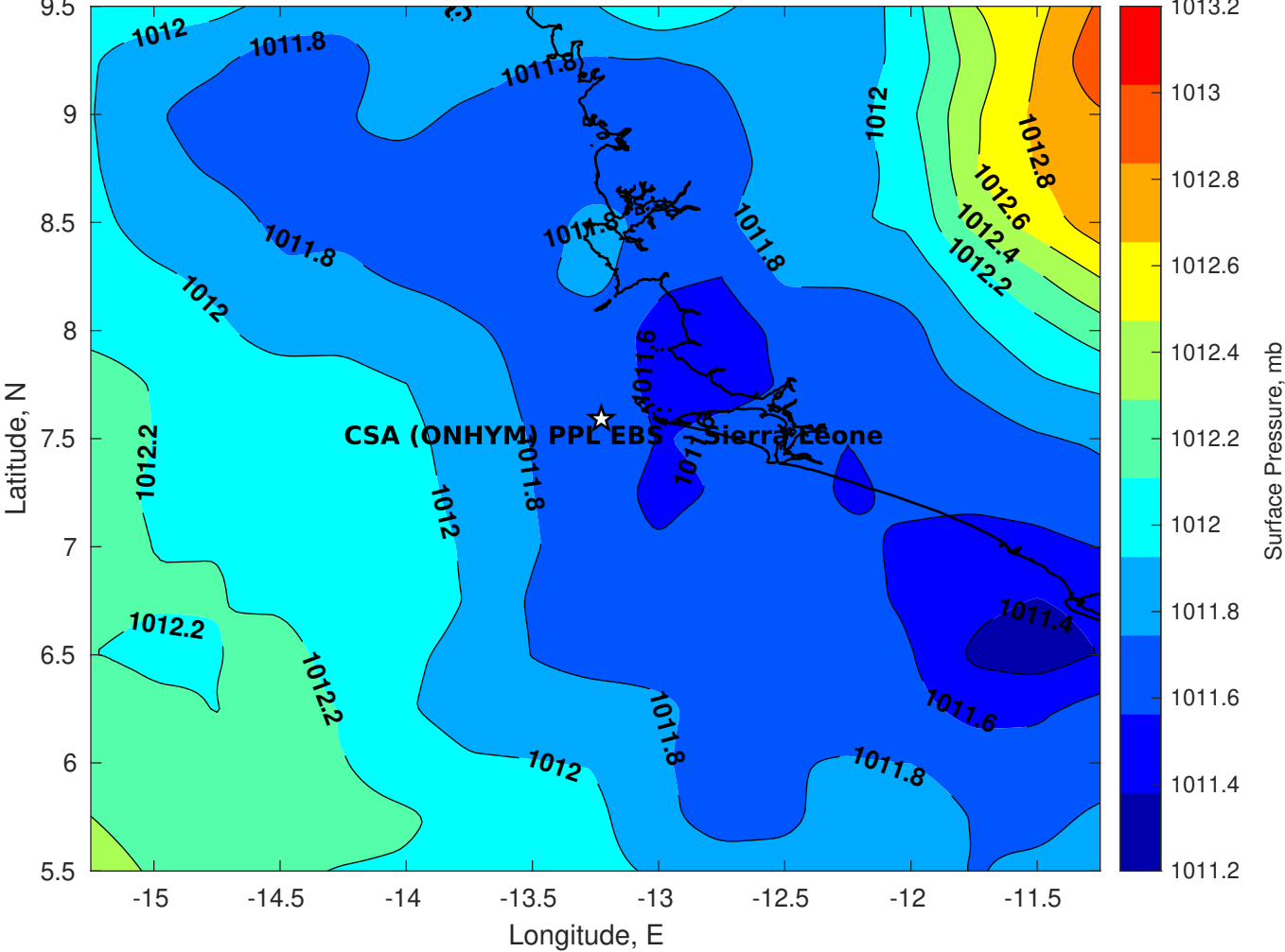
Surface Pressure (mb) for CSA (ONHYM) PPL EBS - Sierra Leone at 06-Dec-2025 00:00:00
