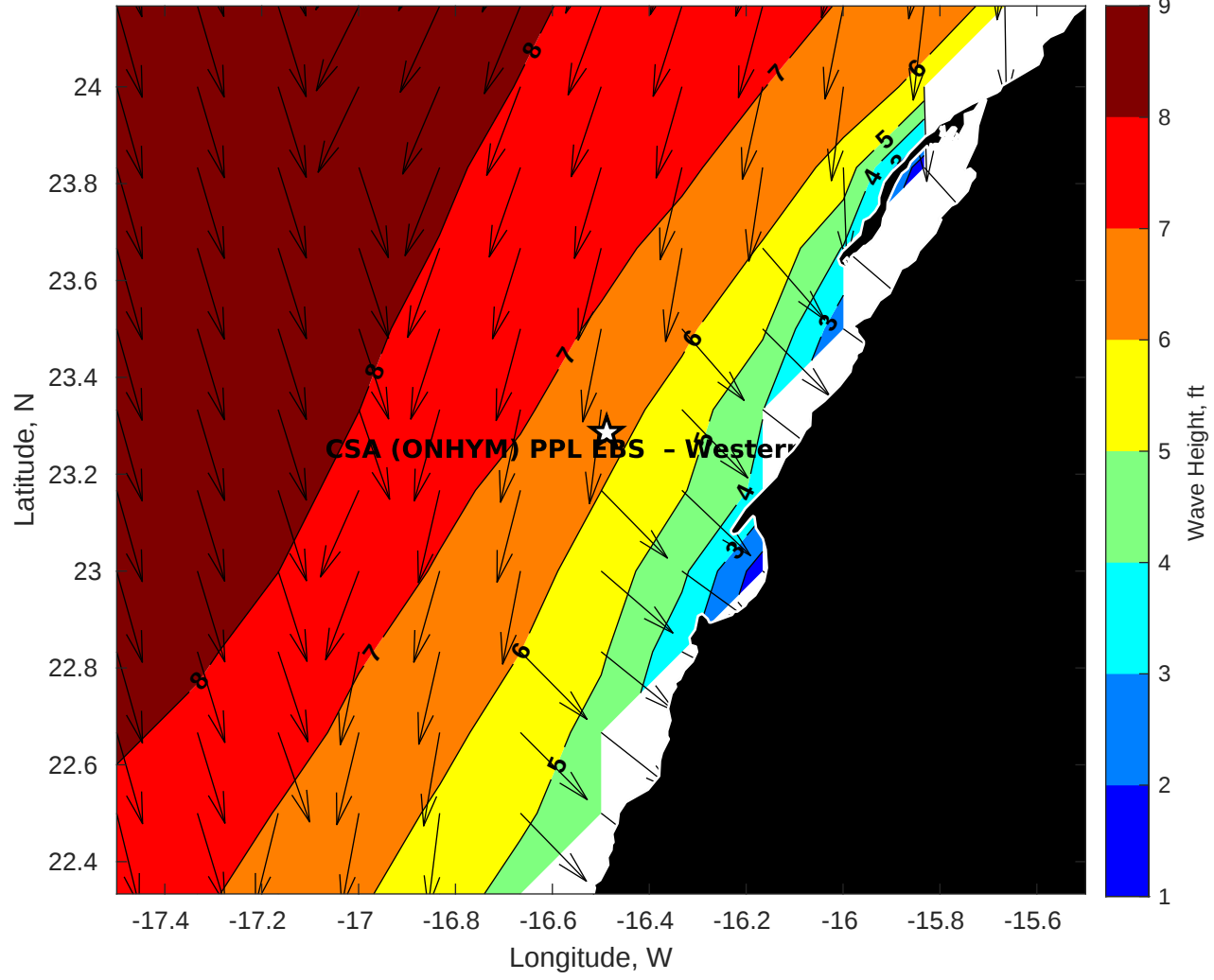
GFS Wave Height (ft) for CSA (ONHYM) PPL EBS - Western Sahara at 04-Dec-2025 09:00:00
