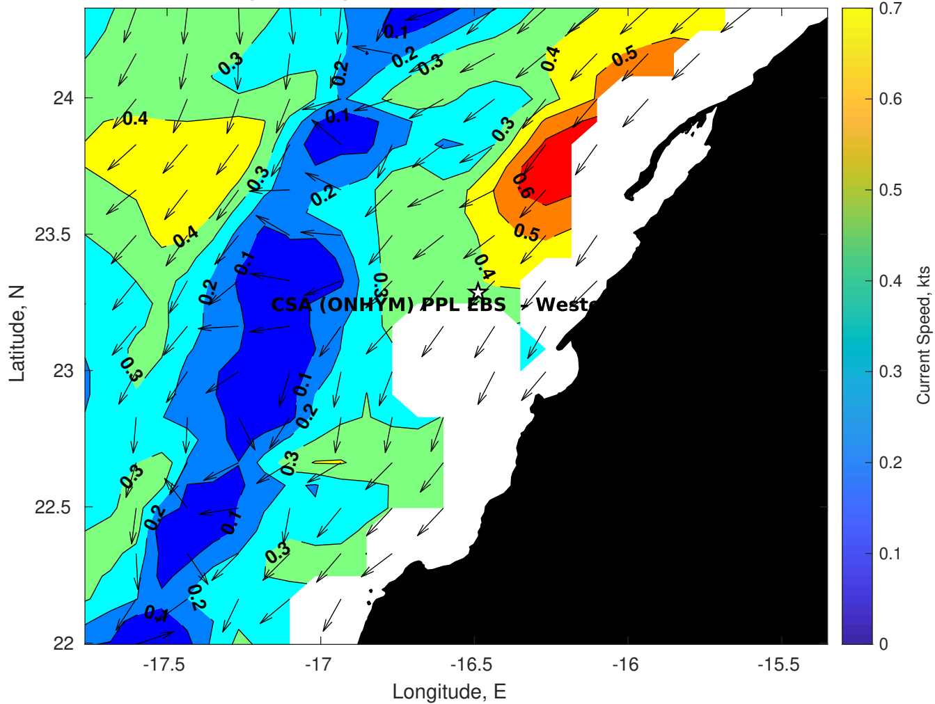
Surface Currents for CSA (ONHYM) PPL EBS - Western Sahara at 03-Dec-2025 00:00:00
