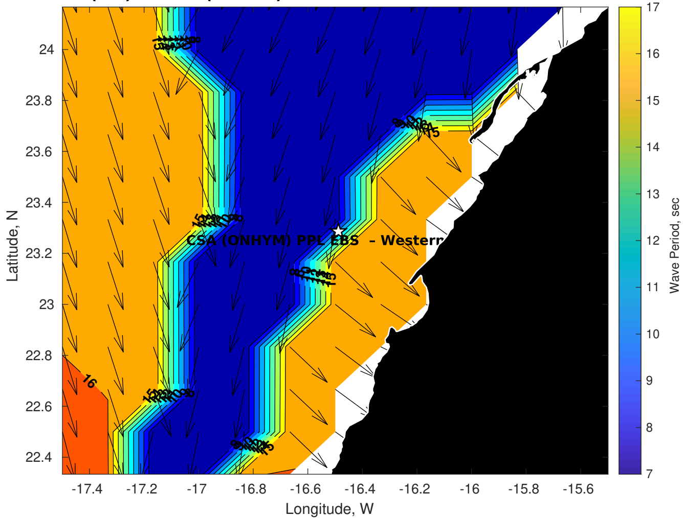
GFS Wave Period (sec) for CSA (ONHYM) PPL EBS - Western Sahara at 04-Dec-2025 09:00:00
