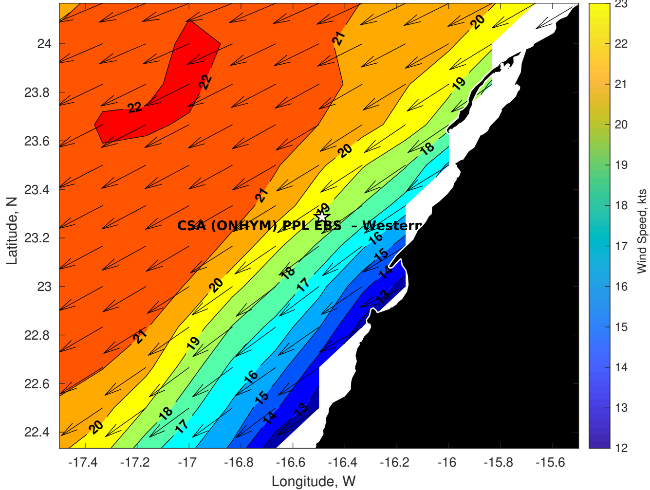
GFS Winds (kts) for CSA (ONHYM) PPL EBS - Western Sahara at 04-Dec-2025 09:00:00
