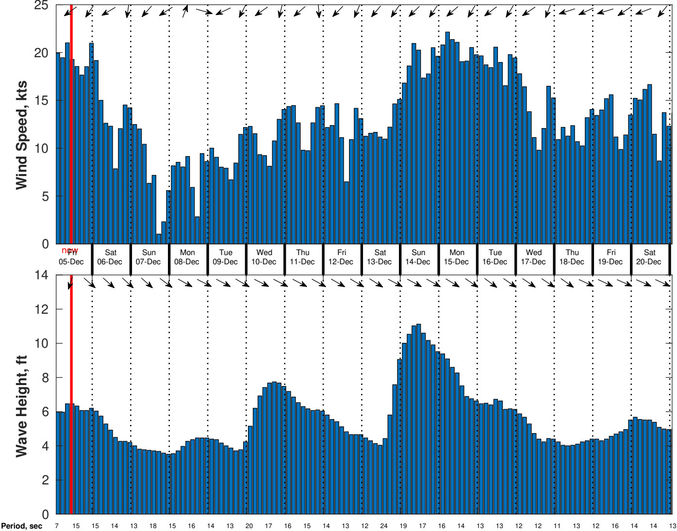
Wind & Wave Forecast for CSA (ONHYM) PPL EBS - Western Sahara from 04-Dec-2025 01:00:00 to 20-Dec-2025 01:00:00
