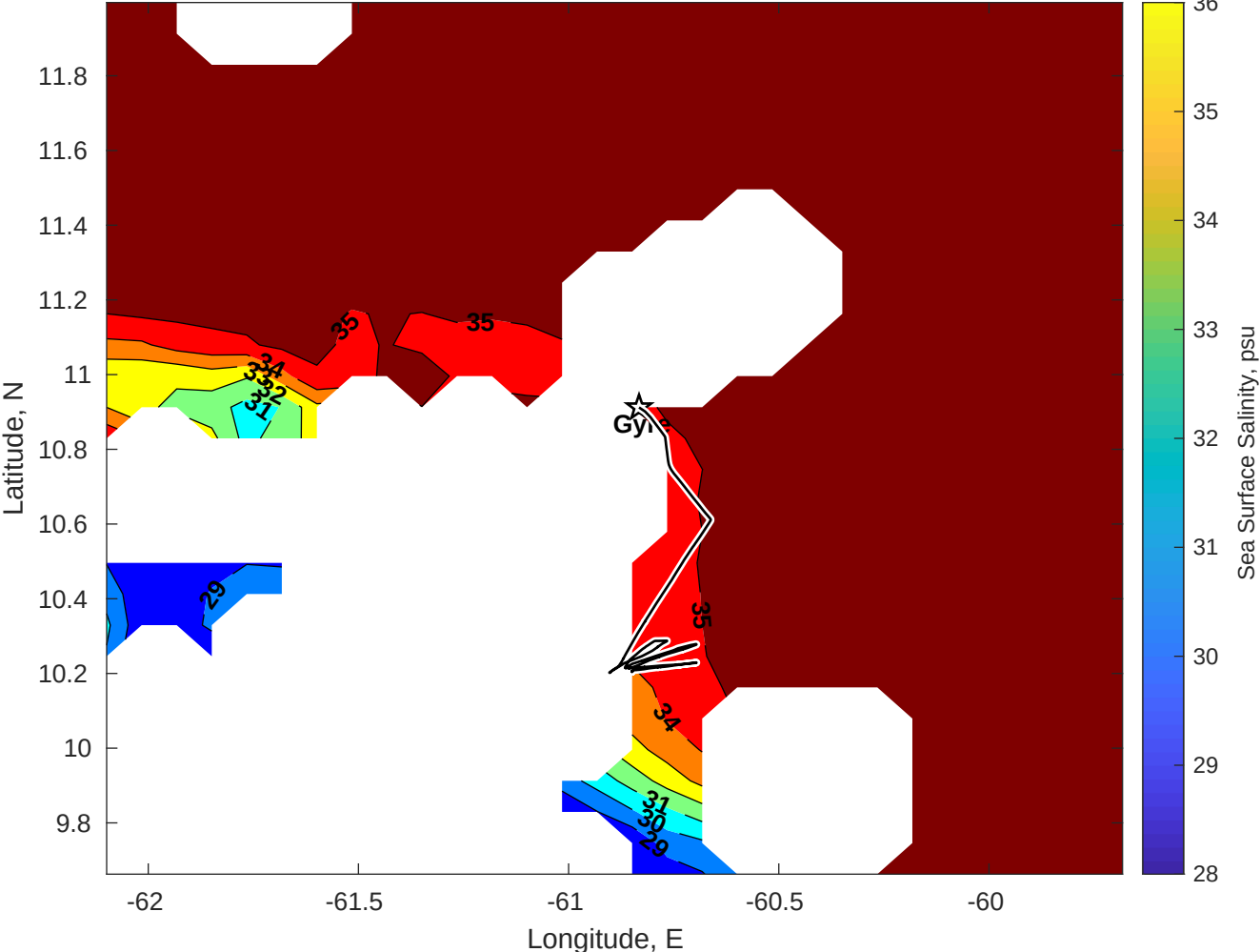
Surface Salinity for Gyre at 03-Dec-2025 00:00:00
