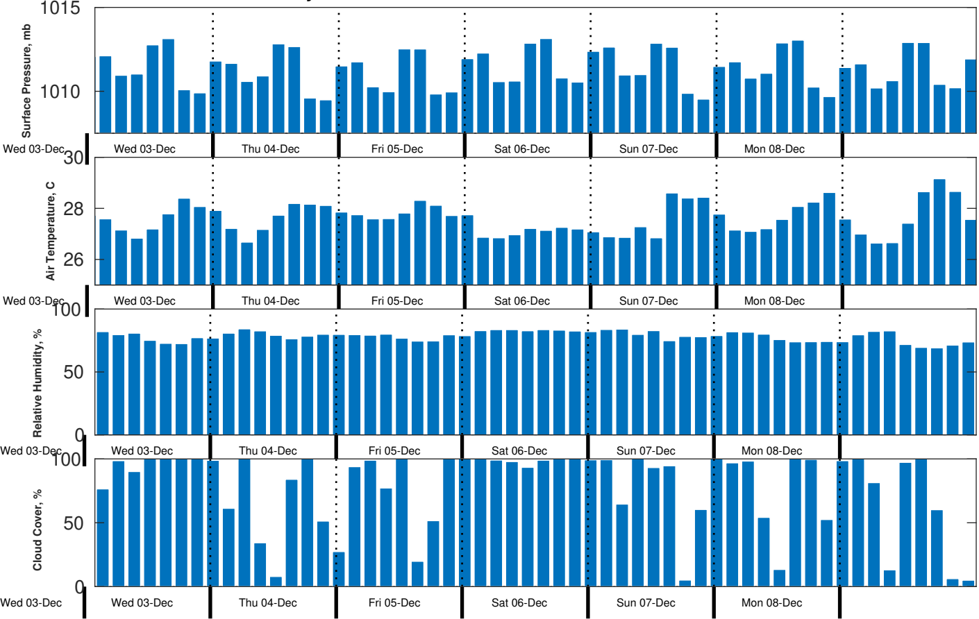
Met Forecast for Gyre from 03-Dec-2025 20:00:00 to 10-Dec-2025 20:00:00
