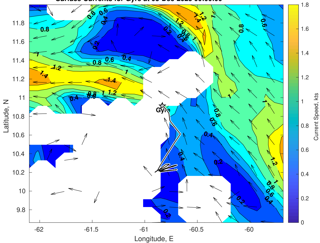
Surface Currents for Gyre at 03-Dec-2025 00:00:00
