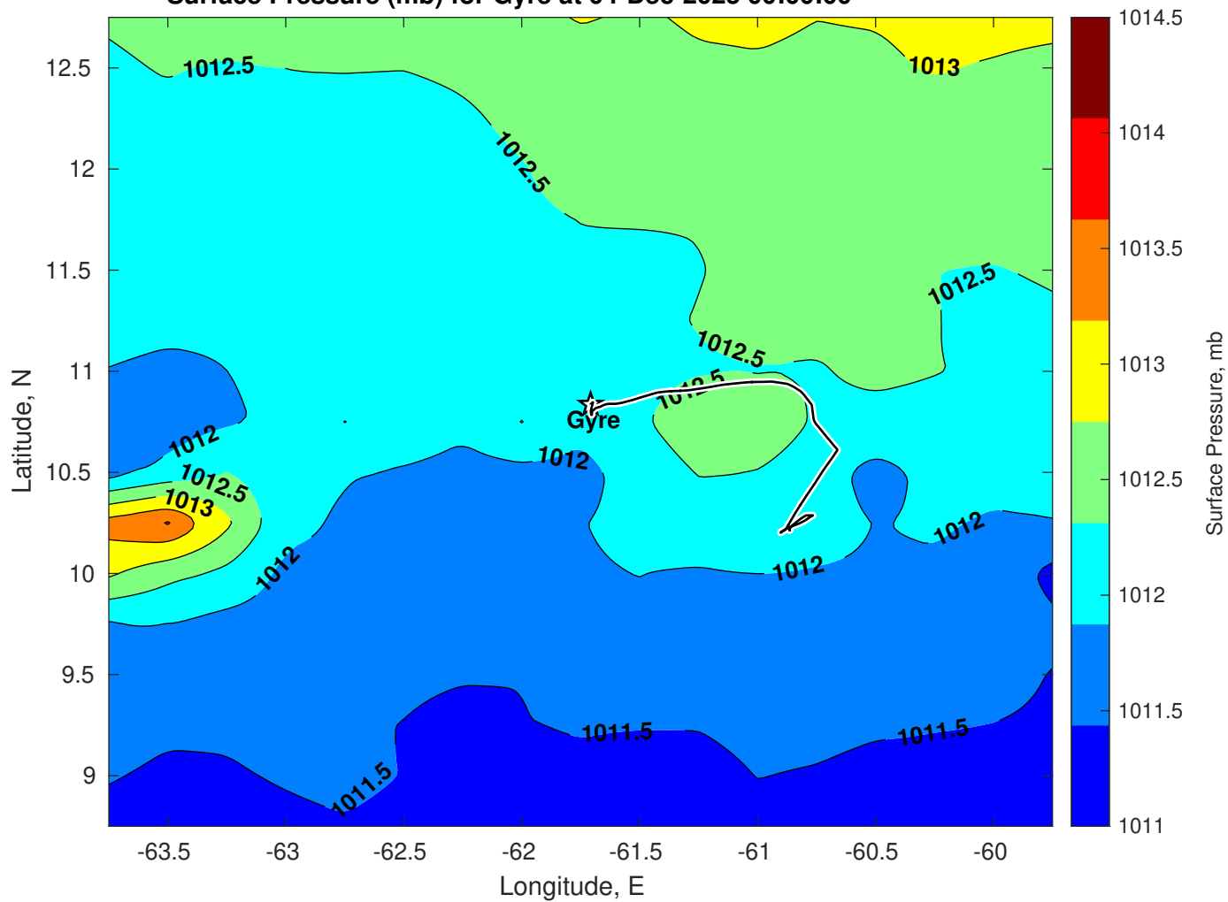
Surface Pressure (mb) for Gyre at 04-Dec-2025 00:00:00
