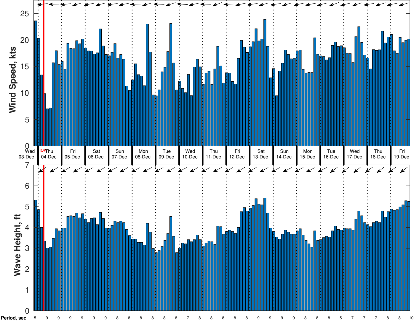
Wind & Wave Forecast for Gyre from 03-Dec-2025 20:00:00 to 19-Dec-2025 20:00:00
