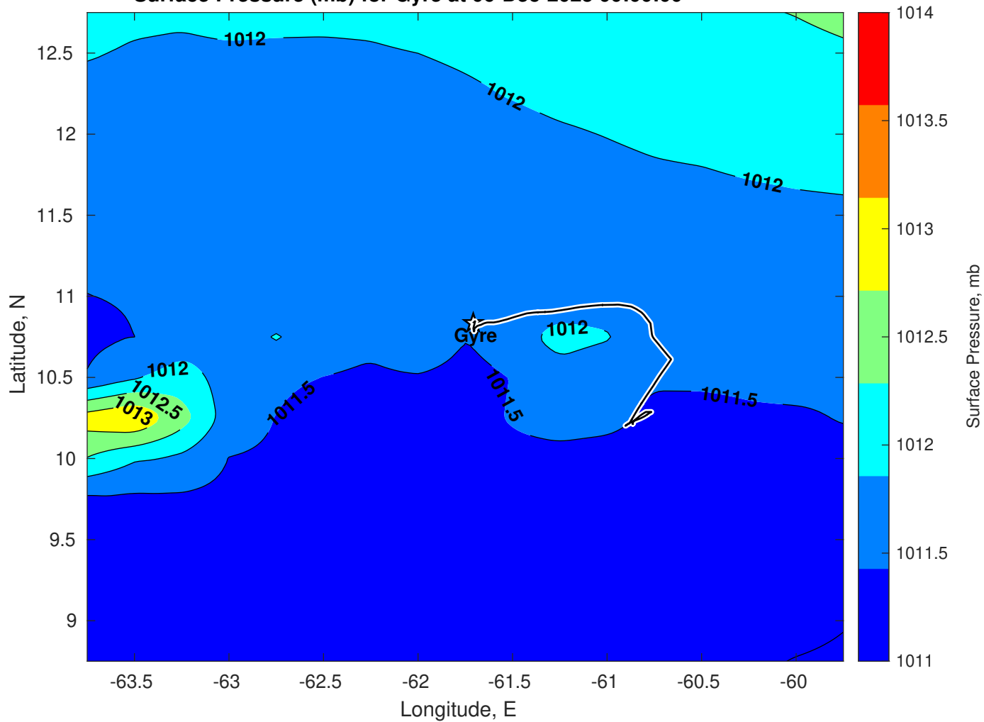
Surface Pressure (mb) for Gyre at 06-Dec-2025 00:00:00
