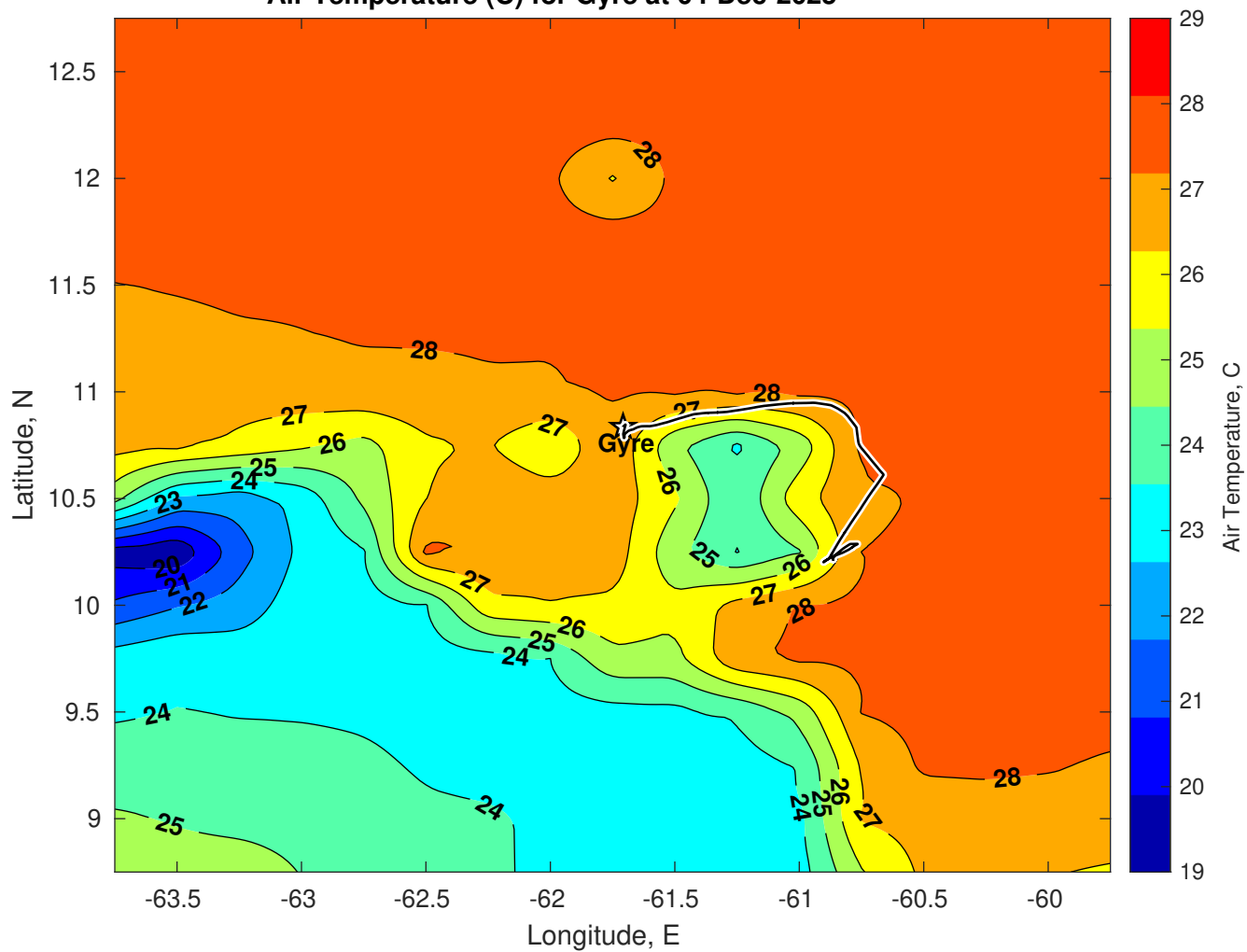
Air Temperature (C) for Gyre at 04-Dec-2025
