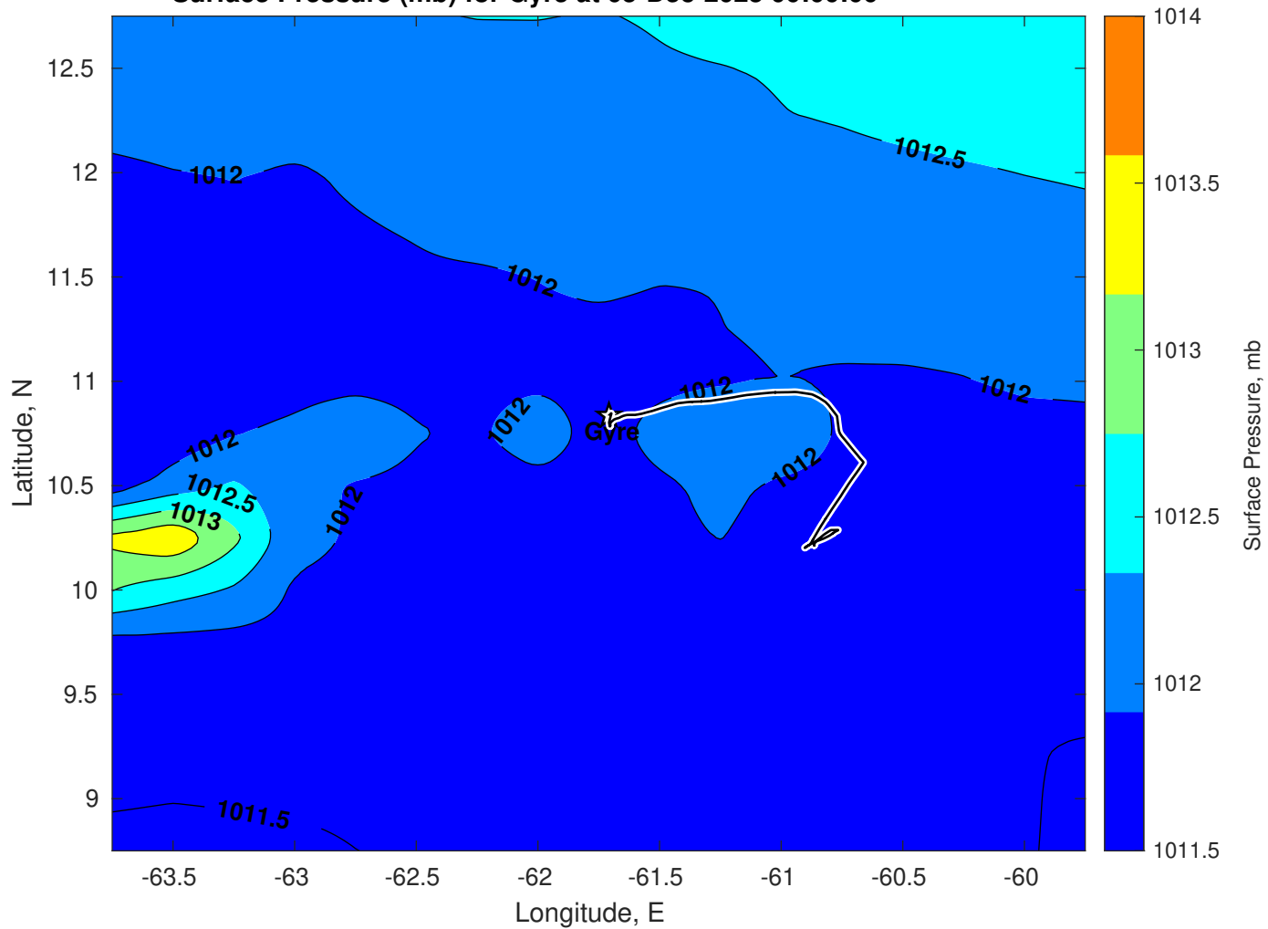
Surface Pressure (mb) for Gyre at 05-Dec-2025 00:00:00
