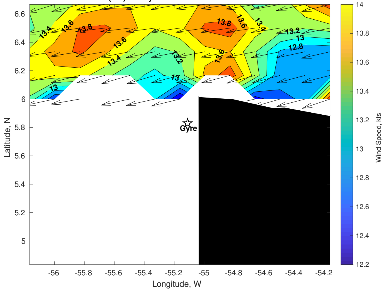
GFS Winds (kts) for Gyre at 27-Nov-2025 09:00:00
