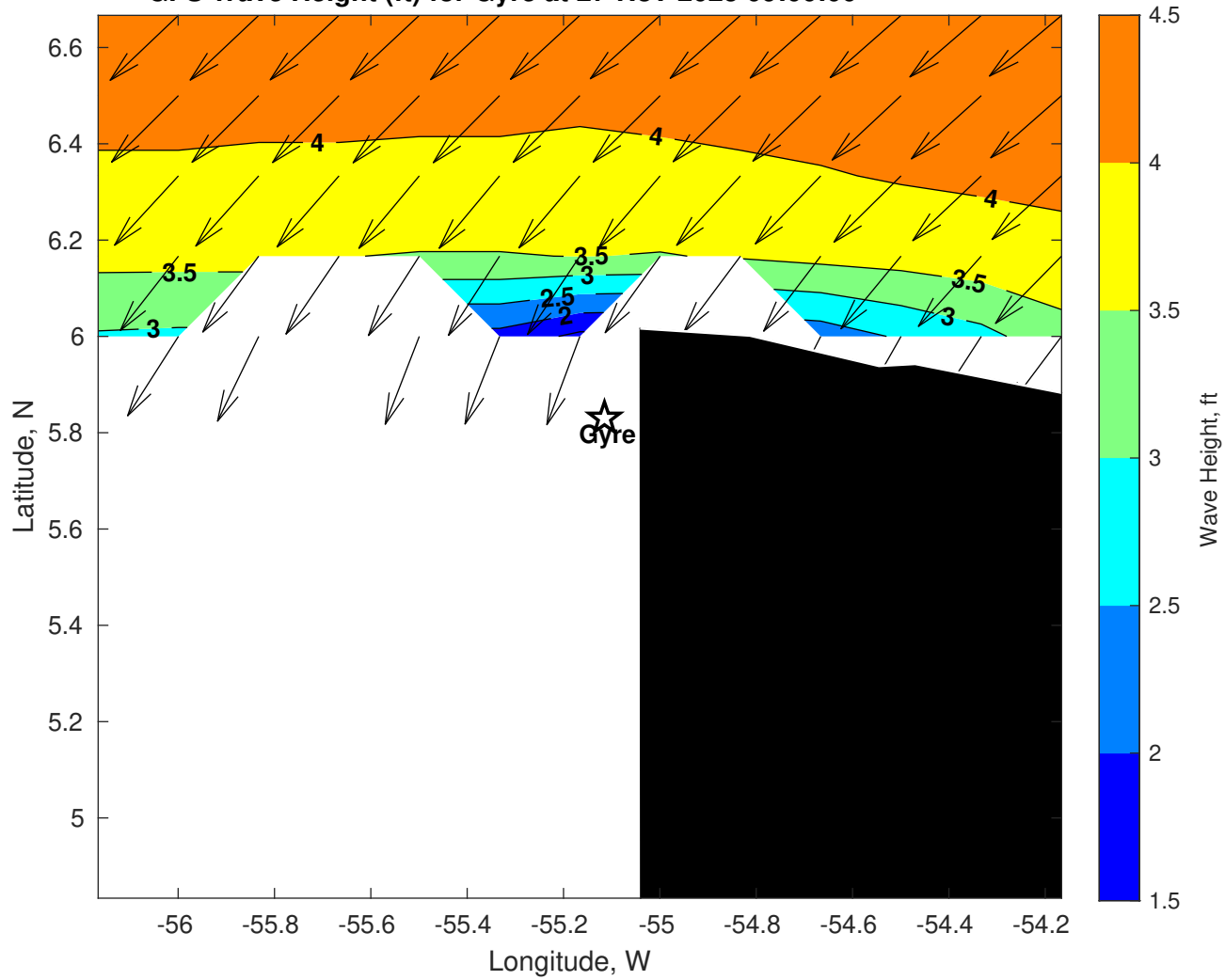
GFS Wave Height (ft) for Gyre at 27-Nov-2025 09:00:00
