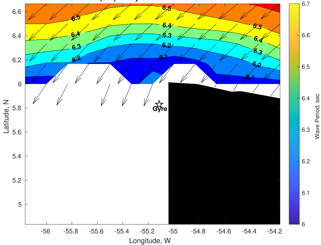
GFS Wave Period (sec) for Gyre at 27-Nov-2025 09:00:00
