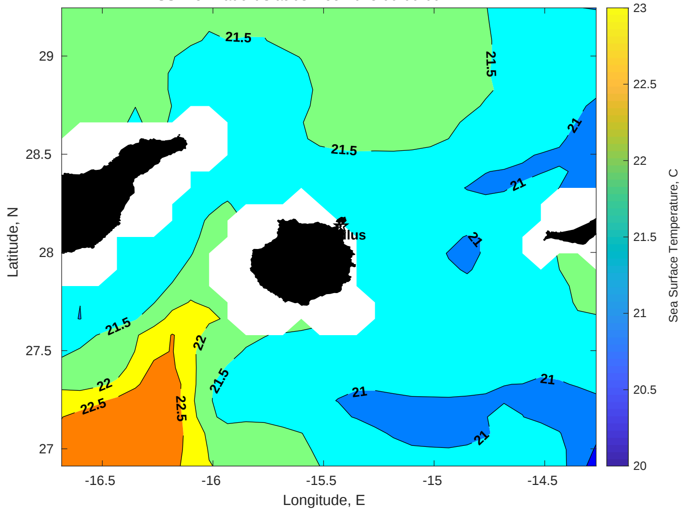
SST for Nautilus at 03-Dec-2025 00:00:00
