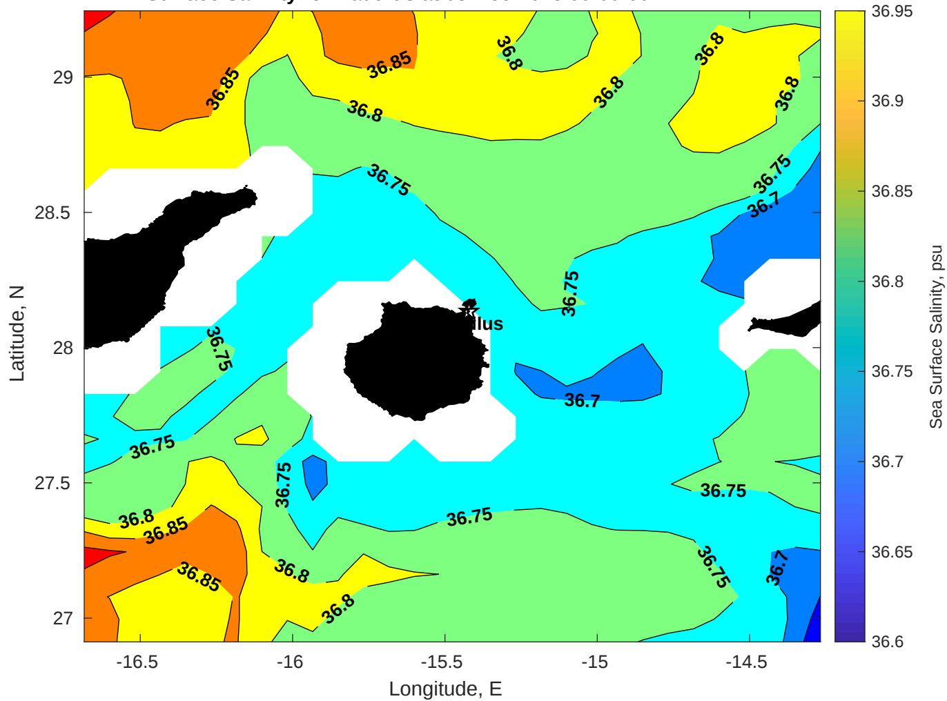
Surface Salinity for Nautilus at 03-Dec-2025 00:00:00
