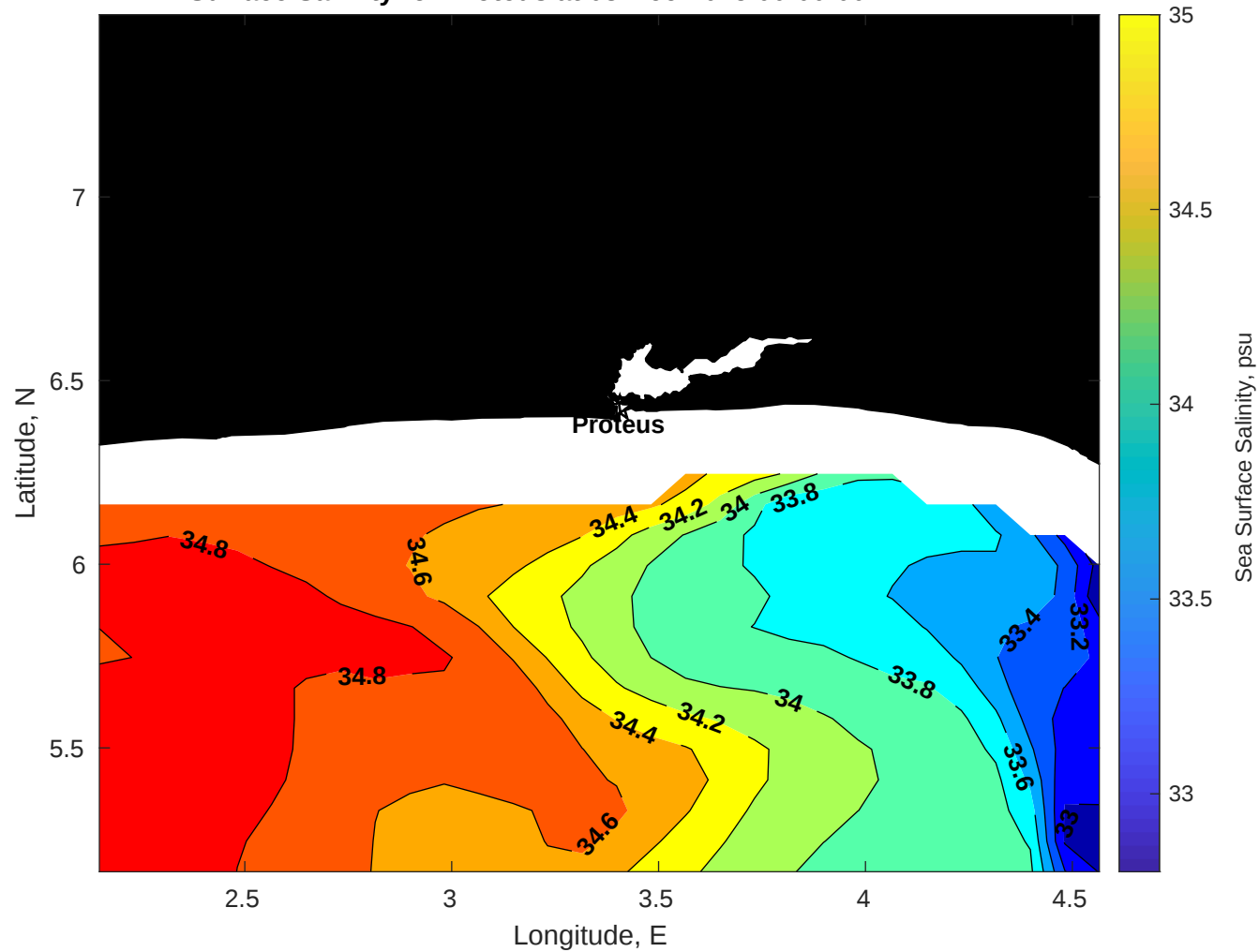
Surface Salinity for Proteus at 03-Dec-2025 00:00:00
