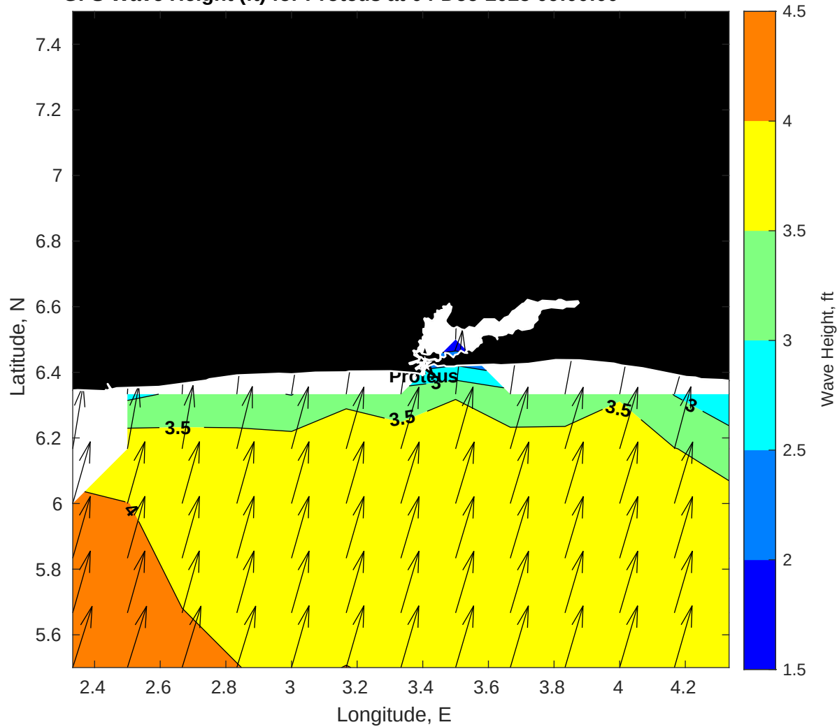
GFS Wave Height (ft) for Proteus at 04-Dec-2025 09:00:00
