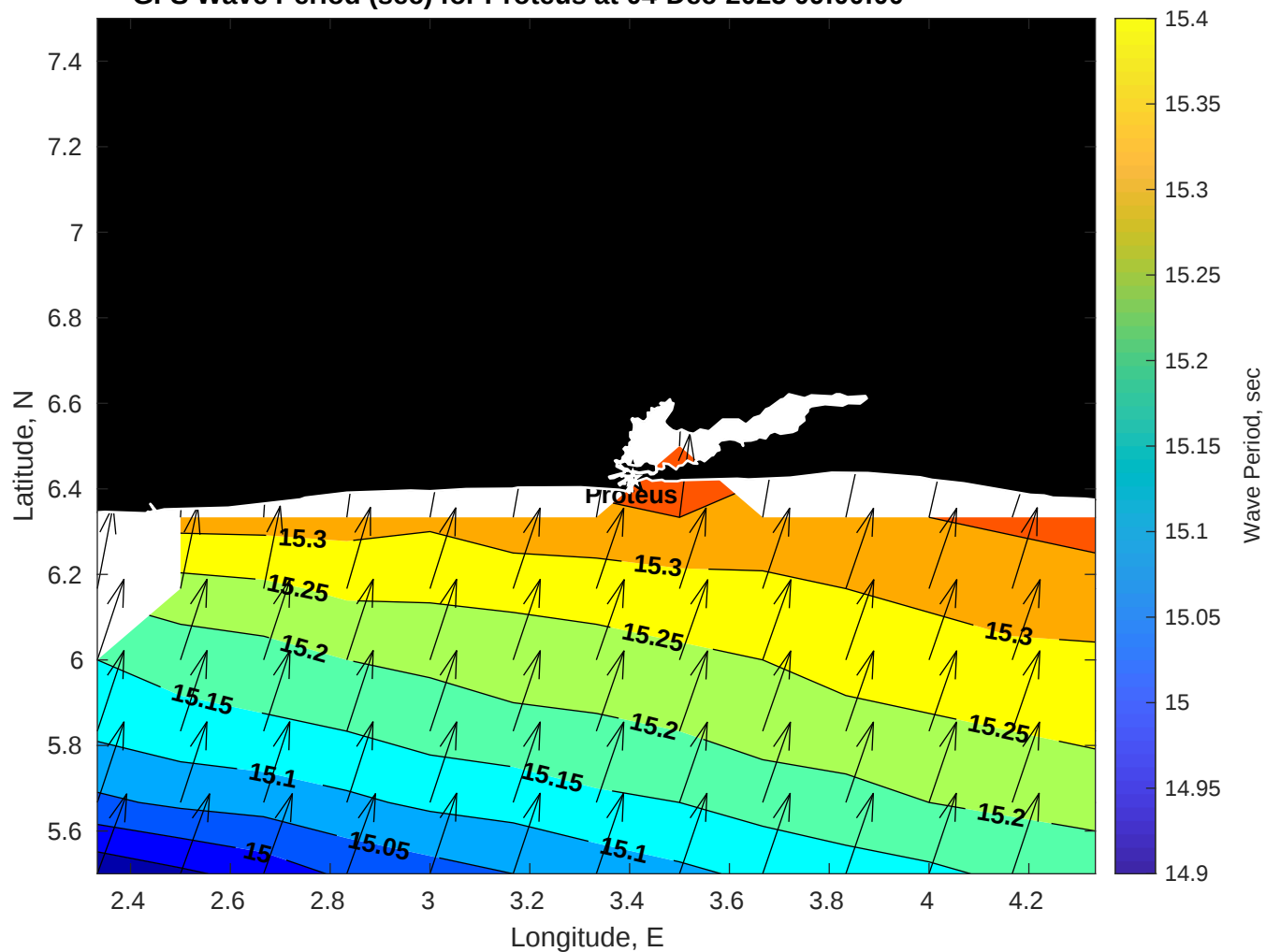
GFS Wave Period (sec) for Proteus at 04-Dec-2025 09:00:00
