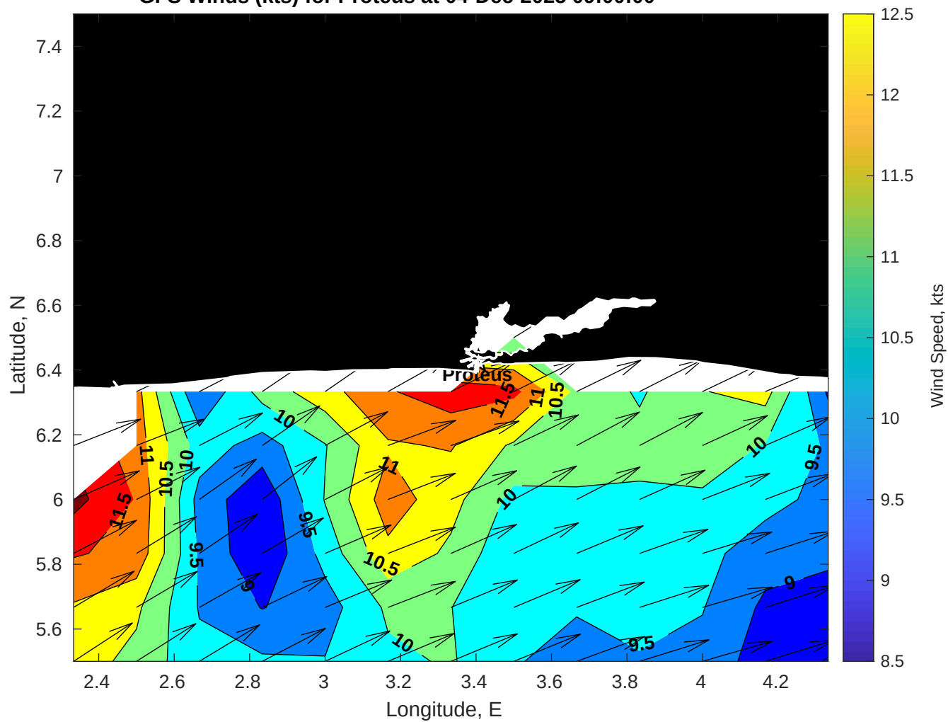
GFS Winds (kts) for Proteus at 04-Dec-2025 09:00:00
