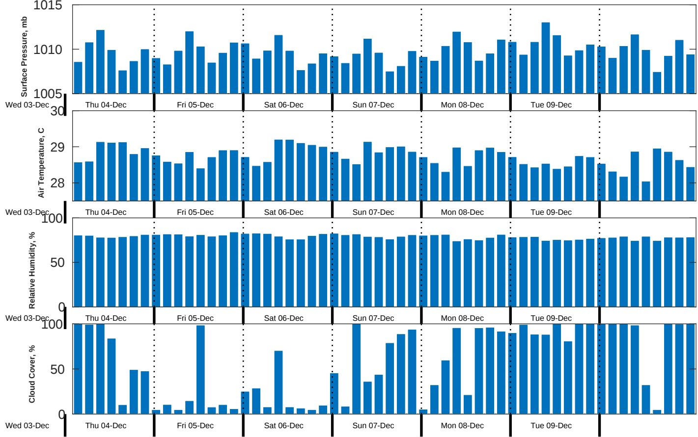
Met Forecast for Proteus from 04-Dec-2025 00:00:00 to 11-Dec-2025 00:00:00
