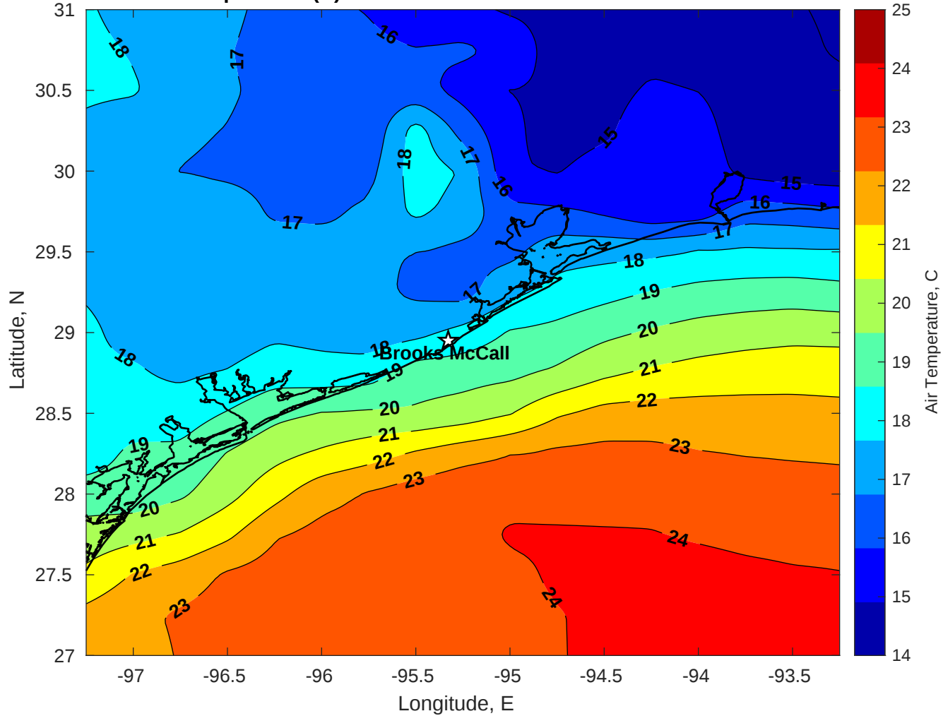
Air Temperature (C) for Brooks McCall at 05-Dec-2025
