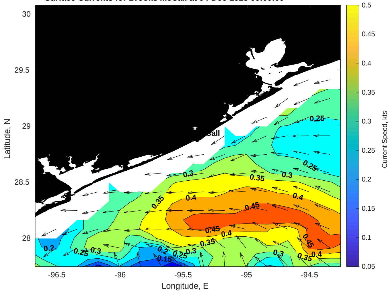
Surface Currents for Brooks McCall at 04-Dec-2025 00:00:00
