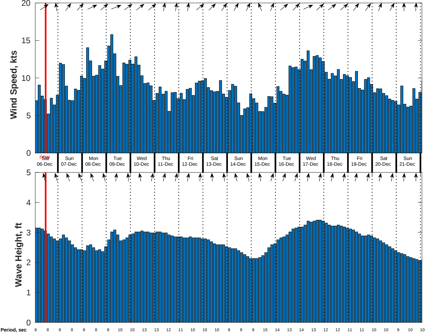
Wind & Wave Forecast for CSA (ONHYM) PPL EBS - Cote d'Ivoire from 05-Dec-2025 01:00:00 to 21-Dec-2025 01:00:00
