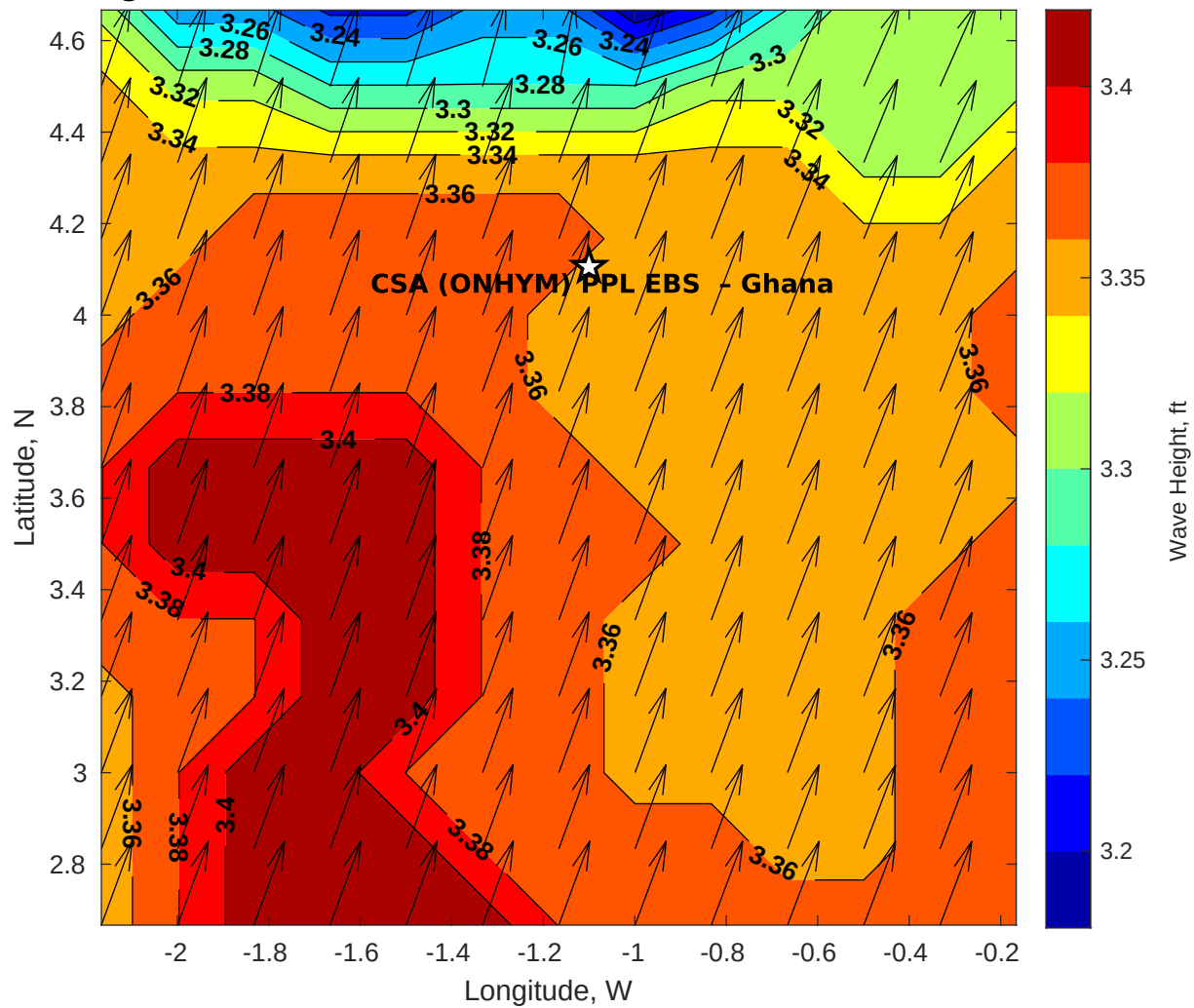
GFS Wave Height (ft) for CSA (ONHYM) PPL EBS - Ghana at 05-Dec-2025 09:00:00
