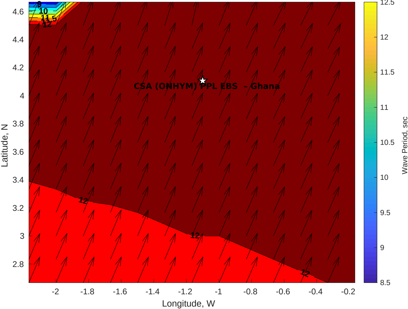
GFS Wave Period (sec) for CSA (ONHYM) PPL EBS - Ghana at 05-Dec-2025 09:00:00
