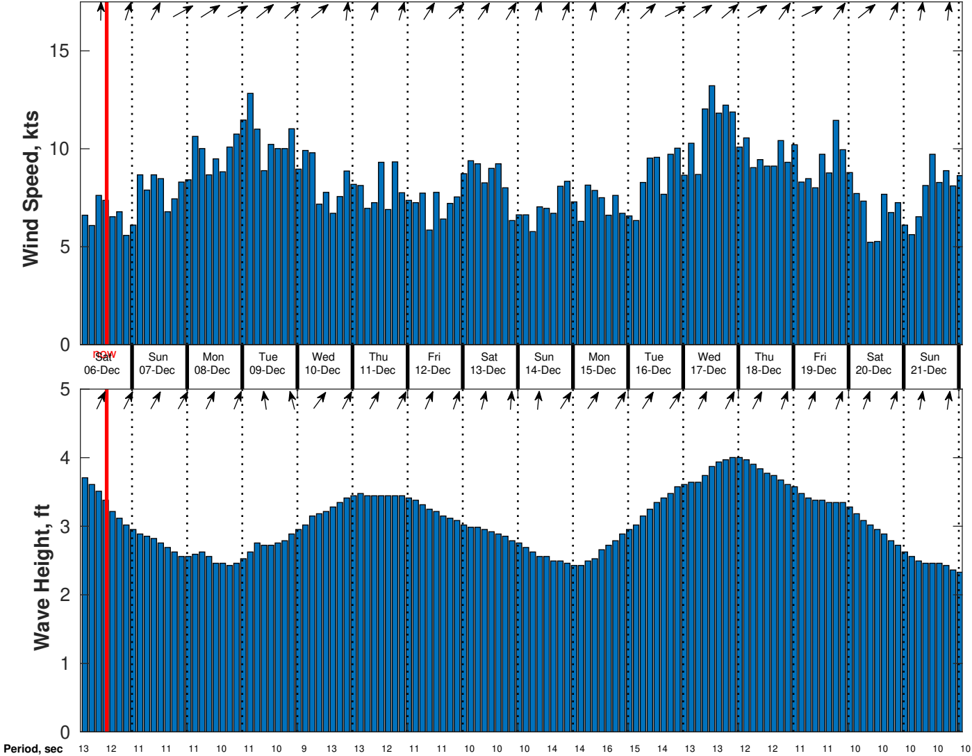
Wind & Wave Forecast for CSA (ONHYM) PPL EBS - Ghana from 05-Dec-2025 02:00:00 to 21-Dec-2025 02:00:00
