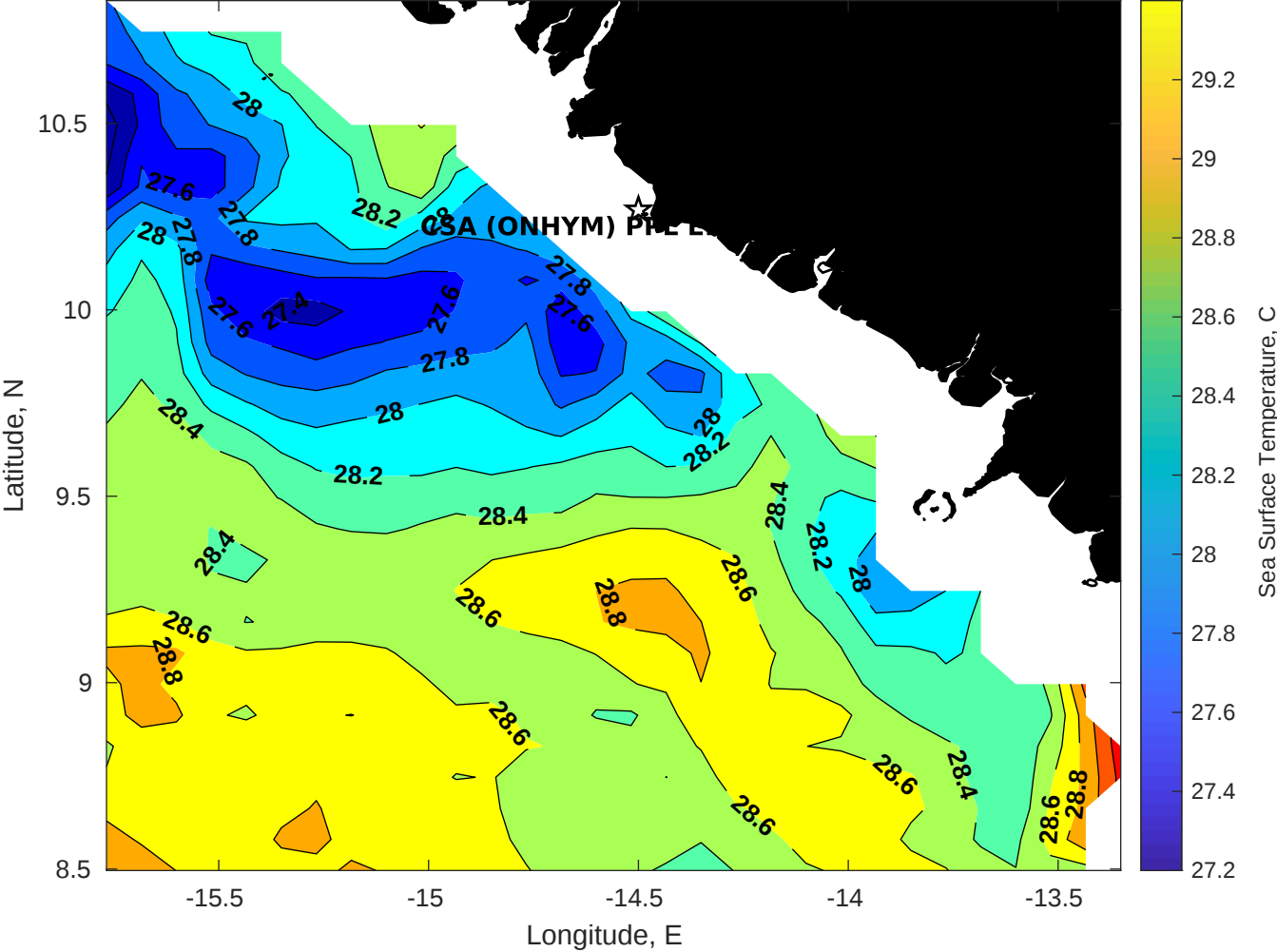
SST for CSA (ONHYM) PPL EBS - Guinea at 04-Dec-2025 00:00:00
