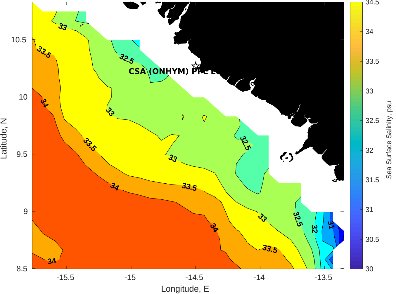
Surface Salinity for CSA (ONHYM) PPL EBS - Guinea at 04-Dec-2025 00:00:00
