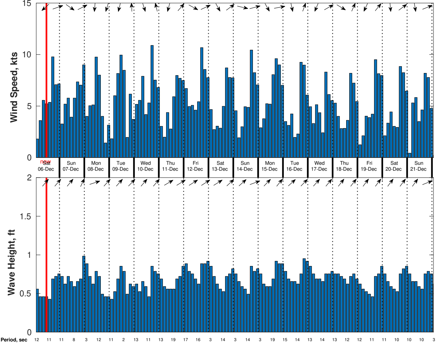
Wind & Wave Forecast for CSA (ONHYM) PPL EBS - Guinea from 05-Dec-2025 01:00:00 to 21-Dec-2025 01:00:00
