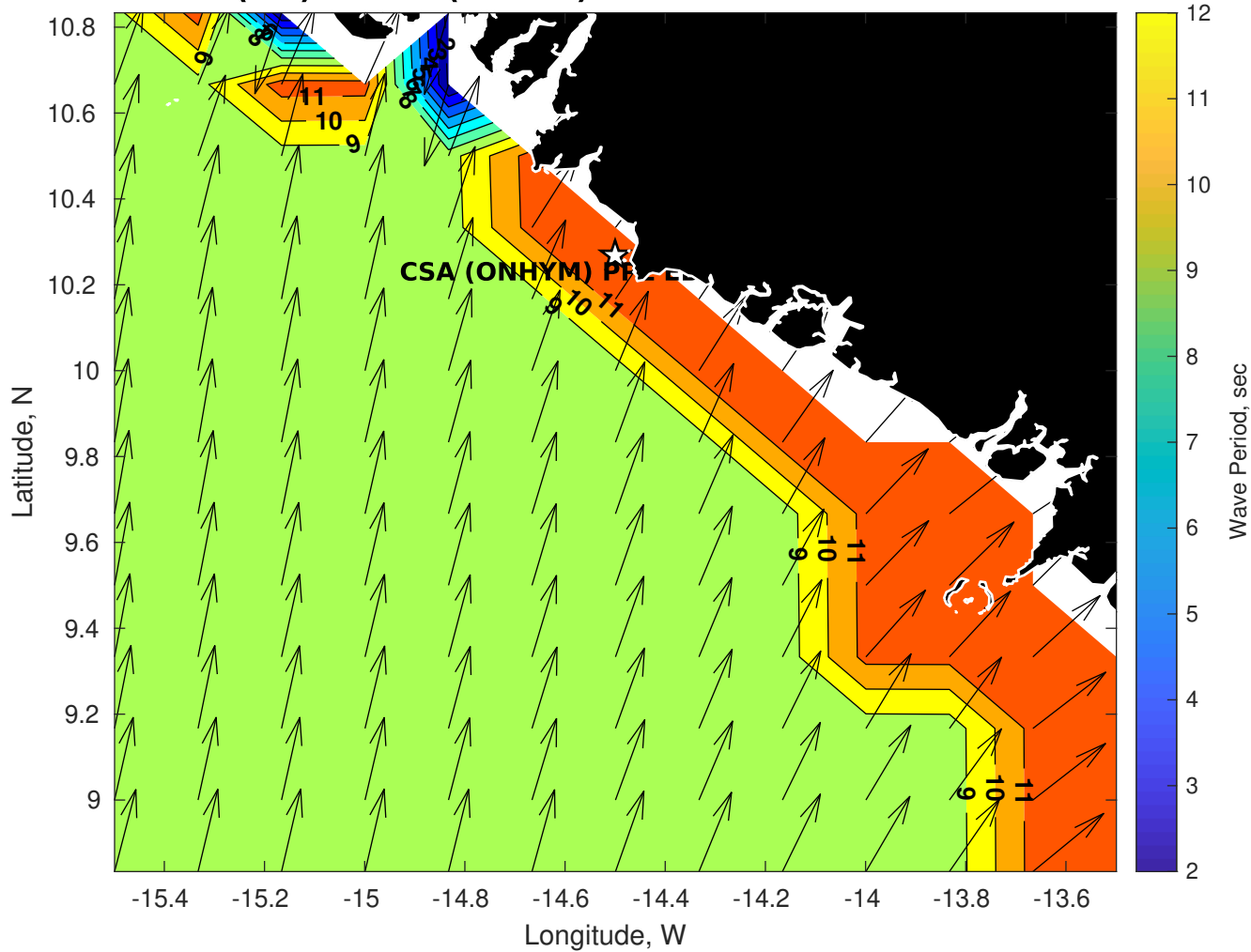
GFS Wave Period (sec) for CSA (ONHYM) PPL EBS - Guinea at 05-Dec-2025 09:00:00
