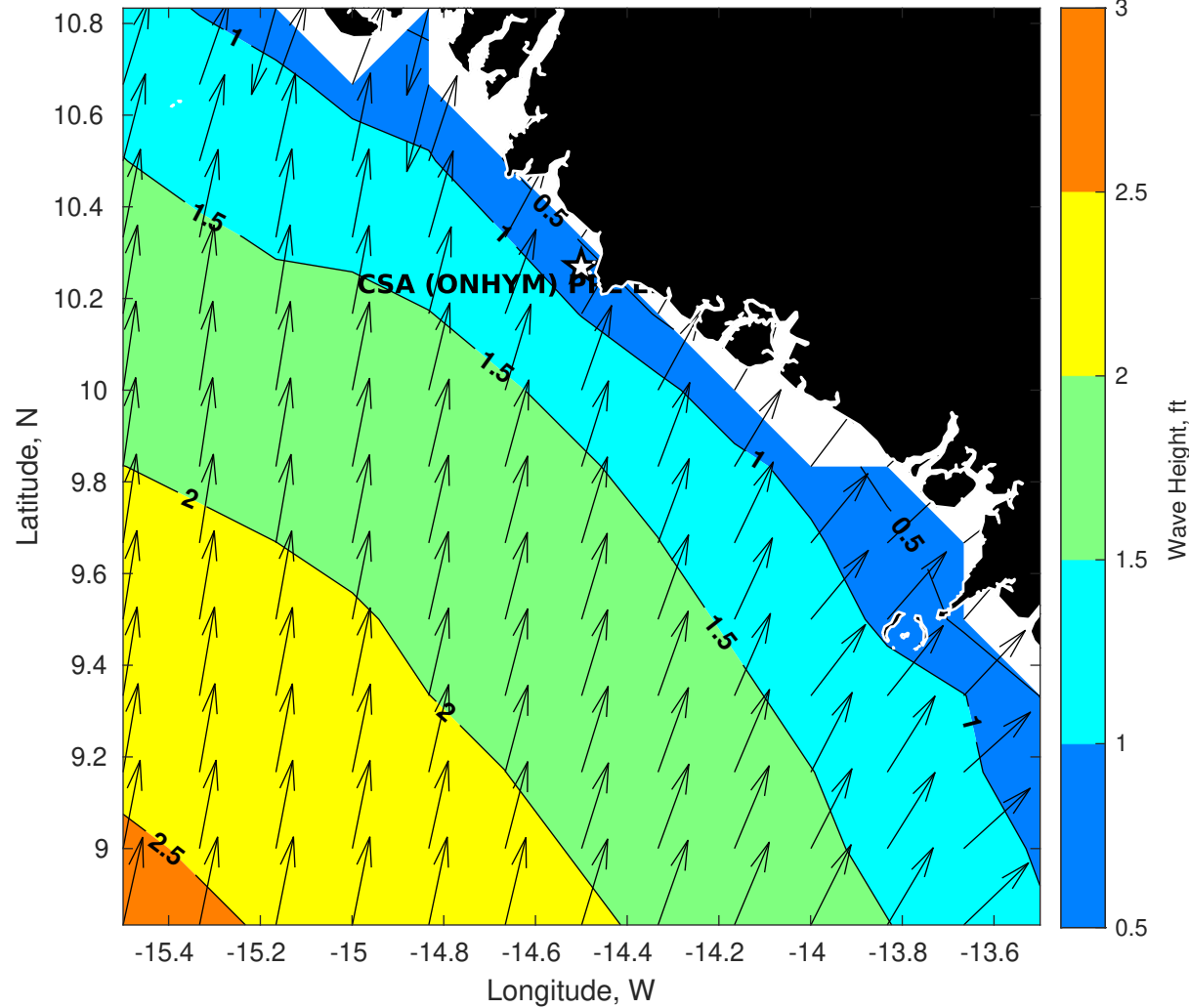
GFS Wave Height (ft) for CSA (ONHYM) PPL EBS - Guinea at 05-Dec-2025 09:00:00
