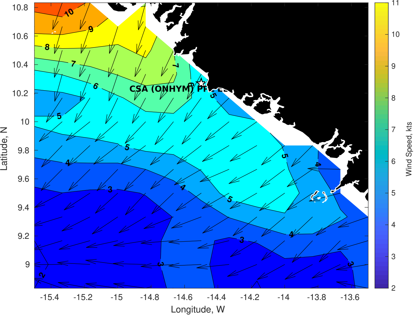
GFS Winds (kts) for CSA (ONHYM) PPL EBS - Guinea at 05-Dec-2025 09:00:00
