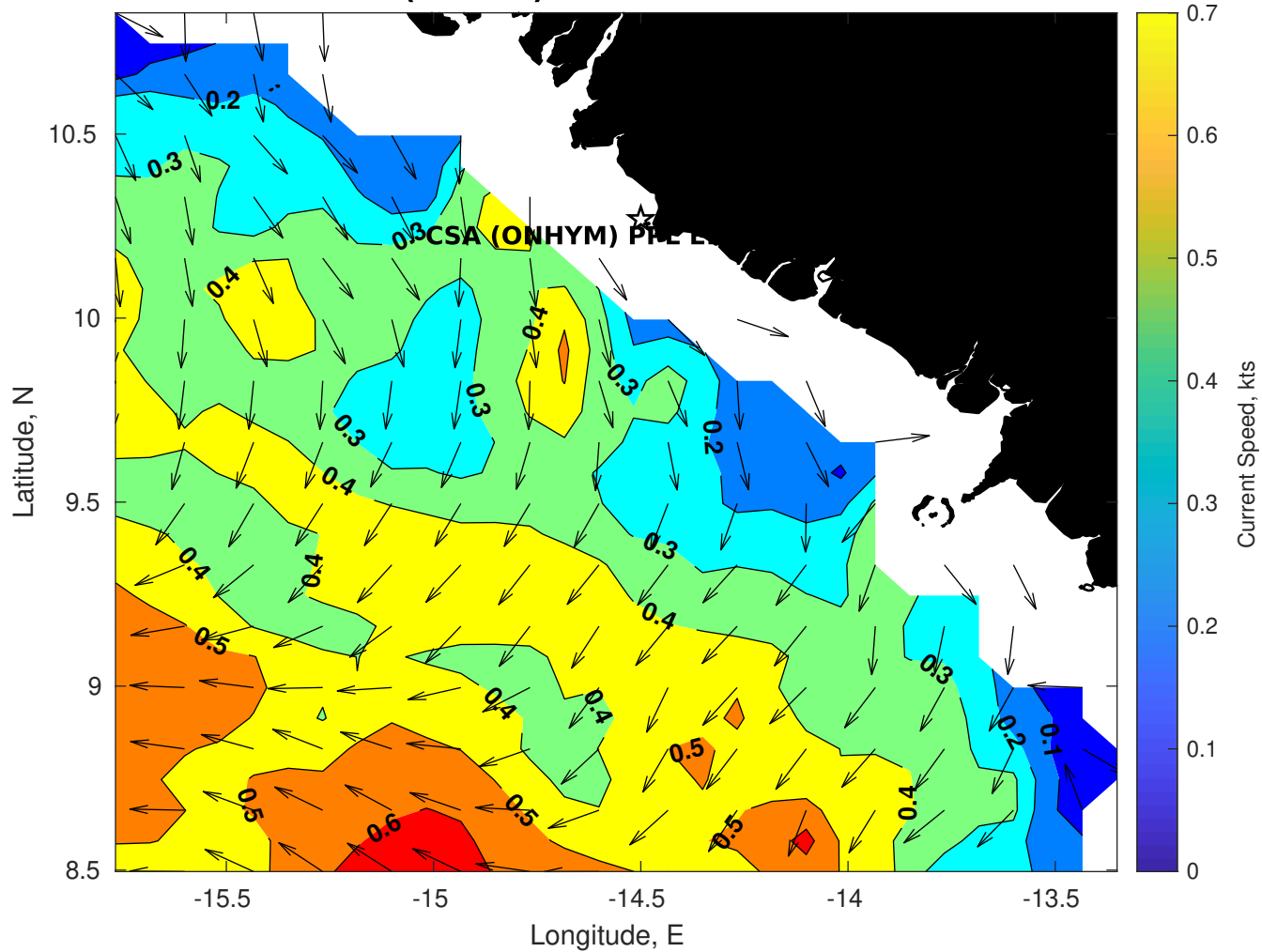
Surface Currents for CSA (ONHYM) PPL EBS - Guinea at 04-Dec-2025 00:00:00
