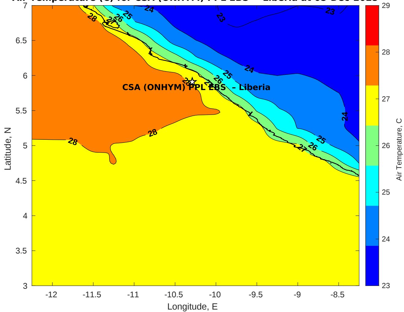
Air Temperature (C) for CSA (ONHYM) PPL EBS - Liberia at 05-Dec-2025
