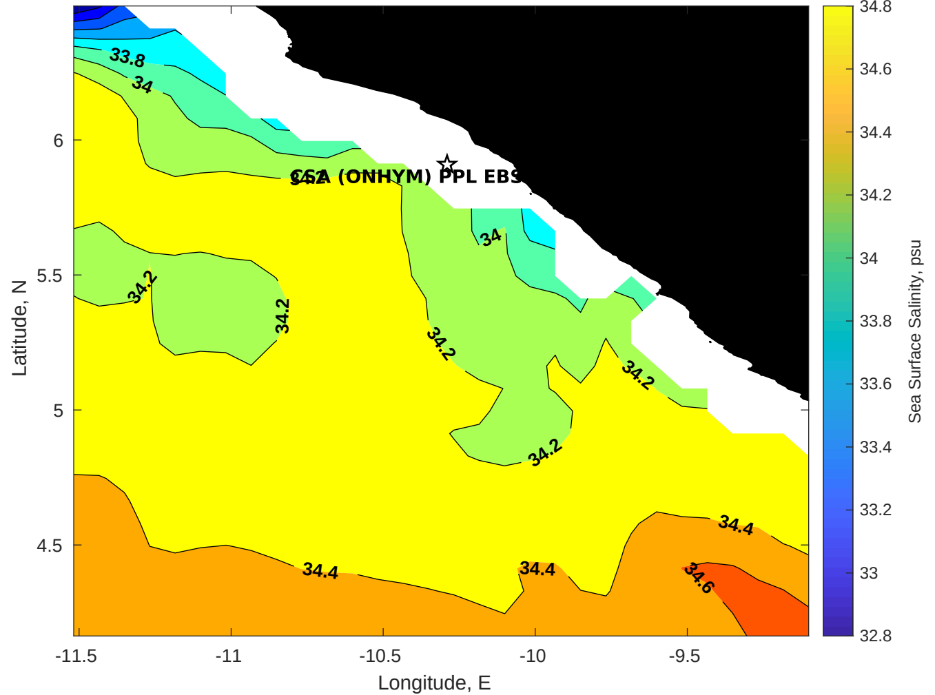
Surface Salinity for CSA (ONHYM) PPL EBS - Liberia at 04-Dec-2025 00:00:00
