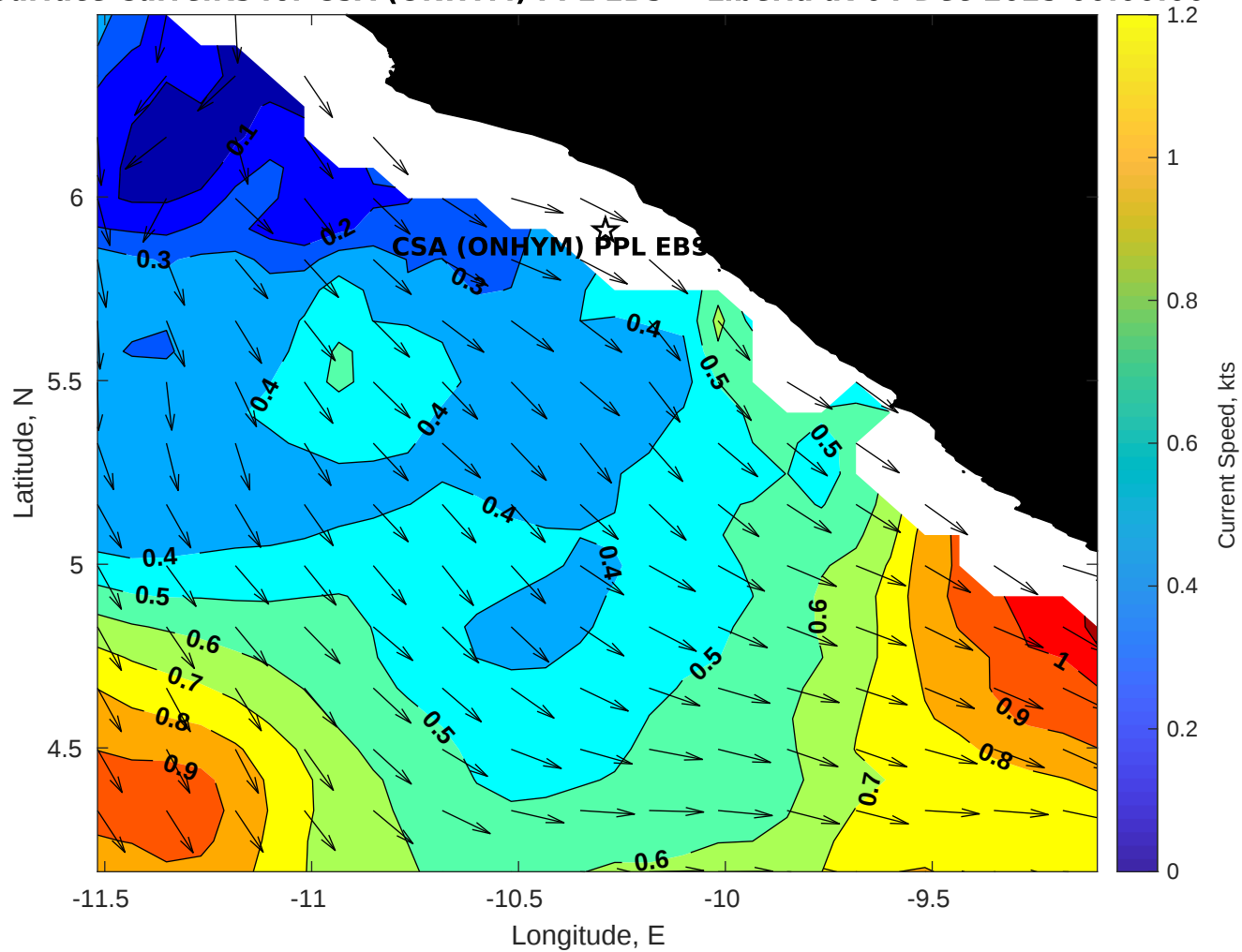
Surface Currents for CSA (ONHYM) PPL EBS - Liberia at 04-Dec-2025 00:00:00
