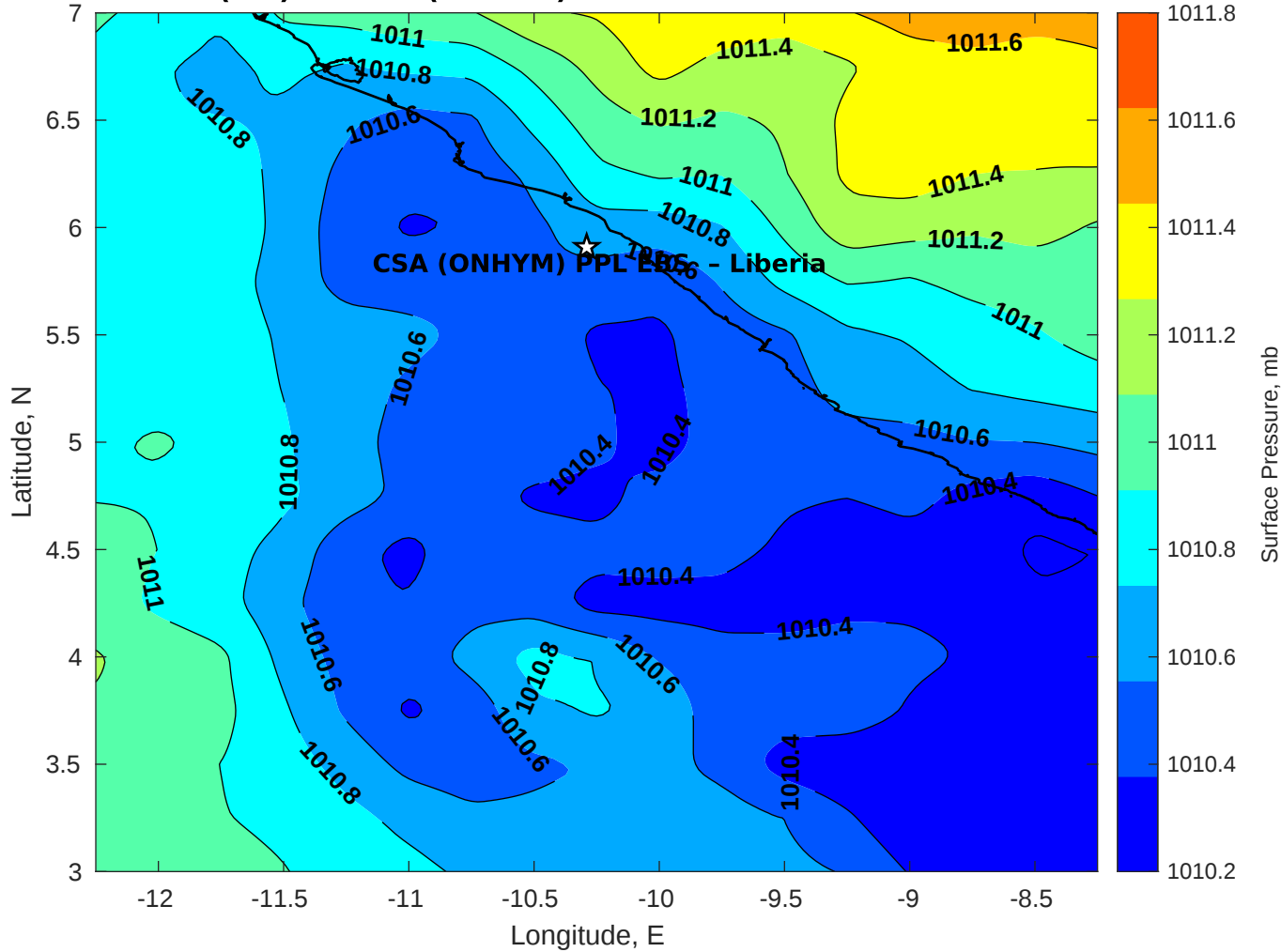
Surface Pressure (mb) for CSA (ONHYM) PPL EBS - Liberia at 05-Dec-2025 00:00:00
