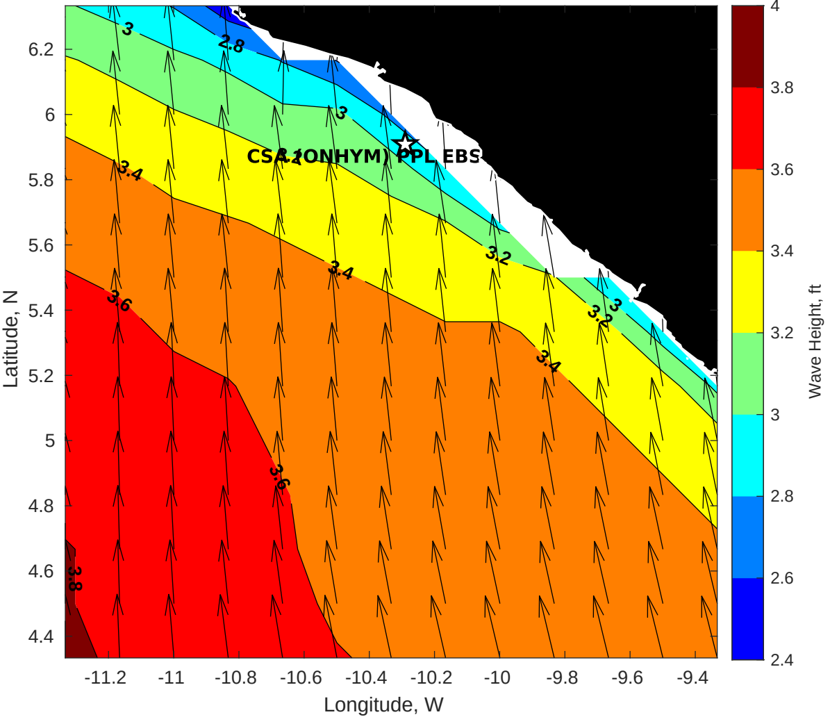
GFS Wave Height (ft) for CSA (ONHYM) PPL EBS - Liberia at 05-Dec-2025 09:00:00
