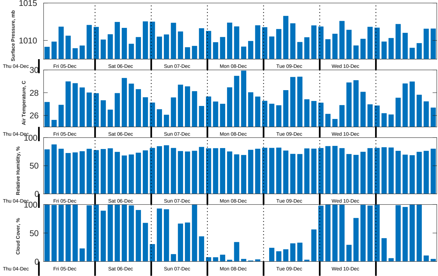
Met Forecast for CSA (ONHYM) PPL EBS - Liberia from 05-Dec-2025 00:00:00 to 12-Dec-2025 00:00:00
