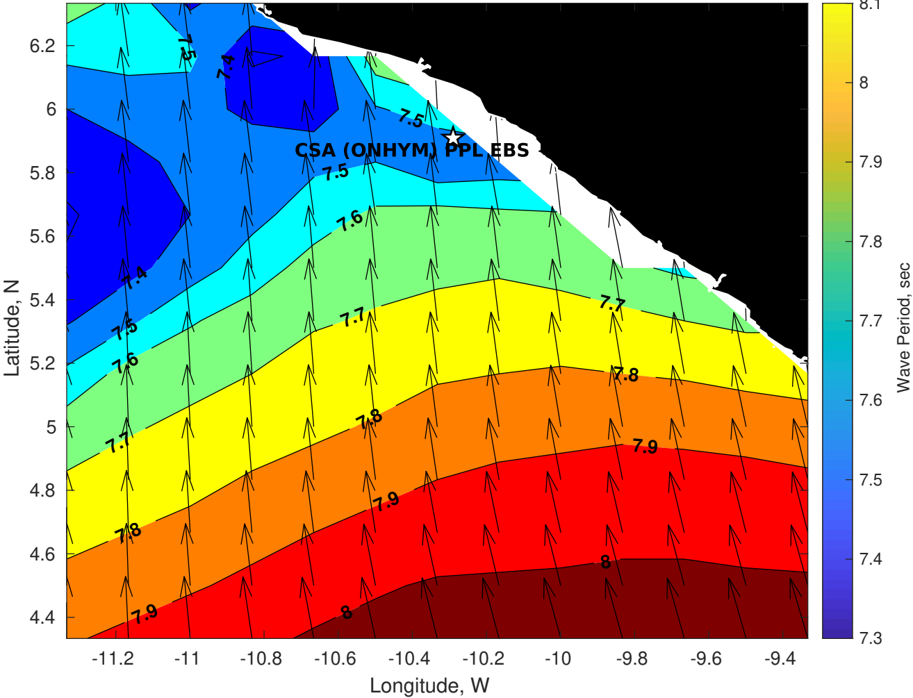
GFS Wave Period (sec) for CSA (ONHYM) PPL EBS - Liberia at 05-Dec-2025 09:00:00
