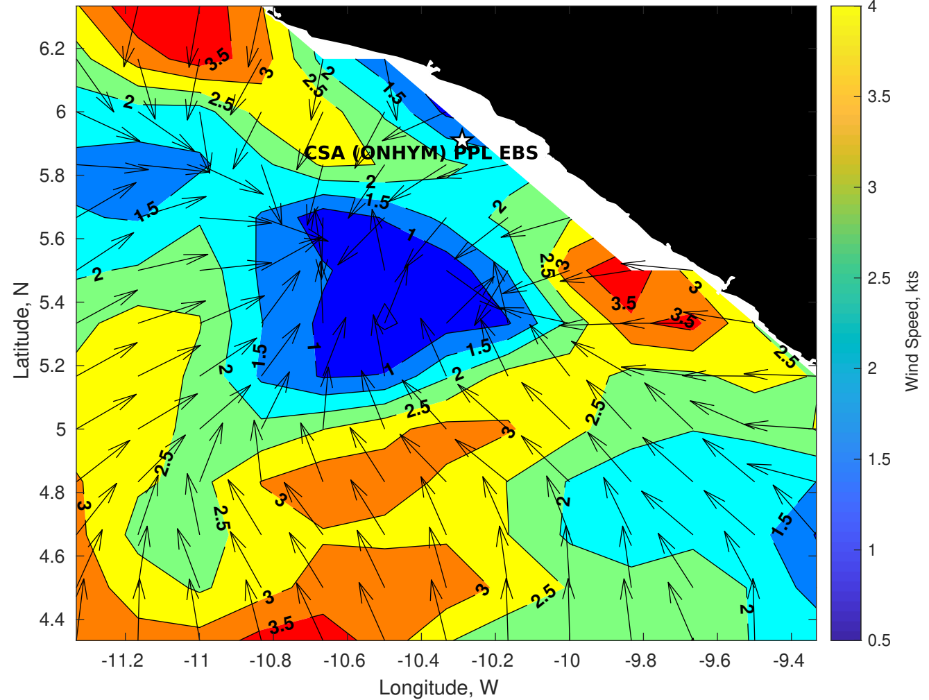
GFS Winds (kts) for CSA (ONHYM) PPL EBS - Liberia at 05-Dec-2025 09:00:00
