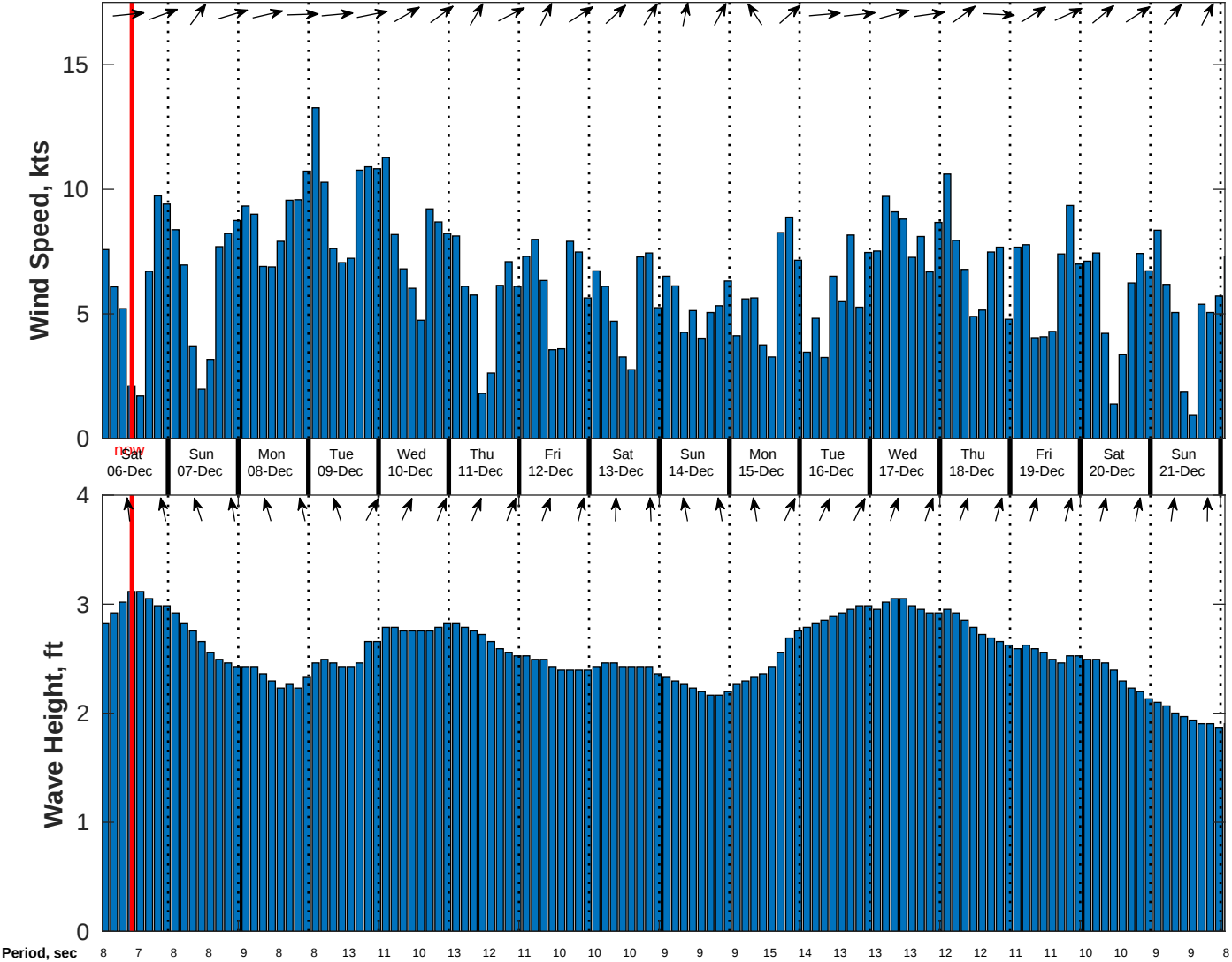
Wind & Wave Forecast for CSA (ONHYM) PPL EBS - Liberia from 05-Dec-2025 01:00:00 to 21-Dec-2025 01:00:00
