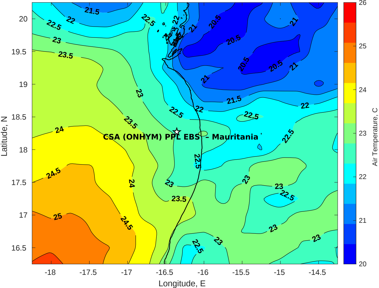
Air Temperature (C) for CSA (ONHYM) PPL EBS - Mauritania at 05-Dec-2025
