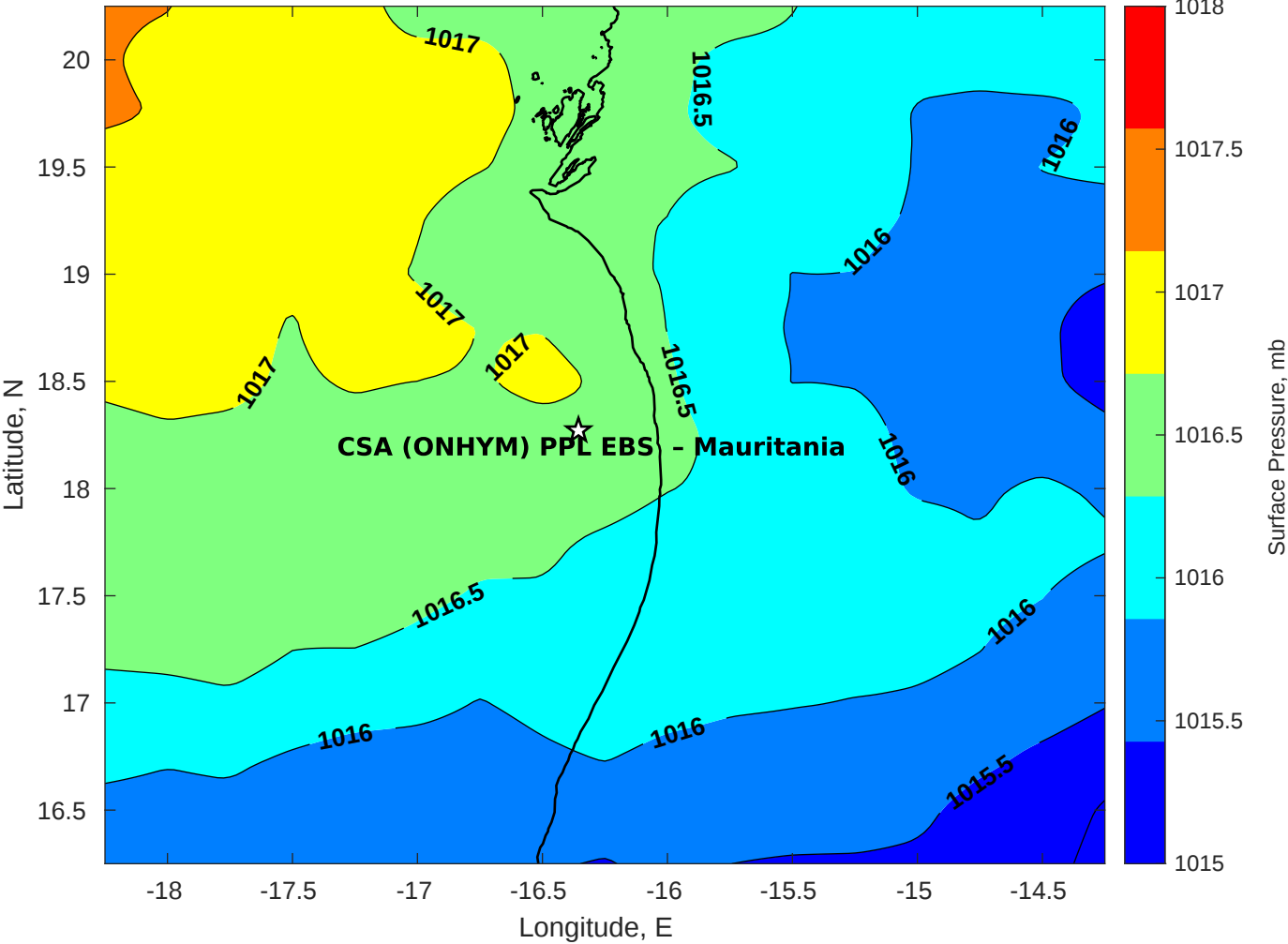
Surface Pressure (mb) for CSA (ONHYM) PPL EBS - Mauritania at 06-Dec-2025 00:00:00
