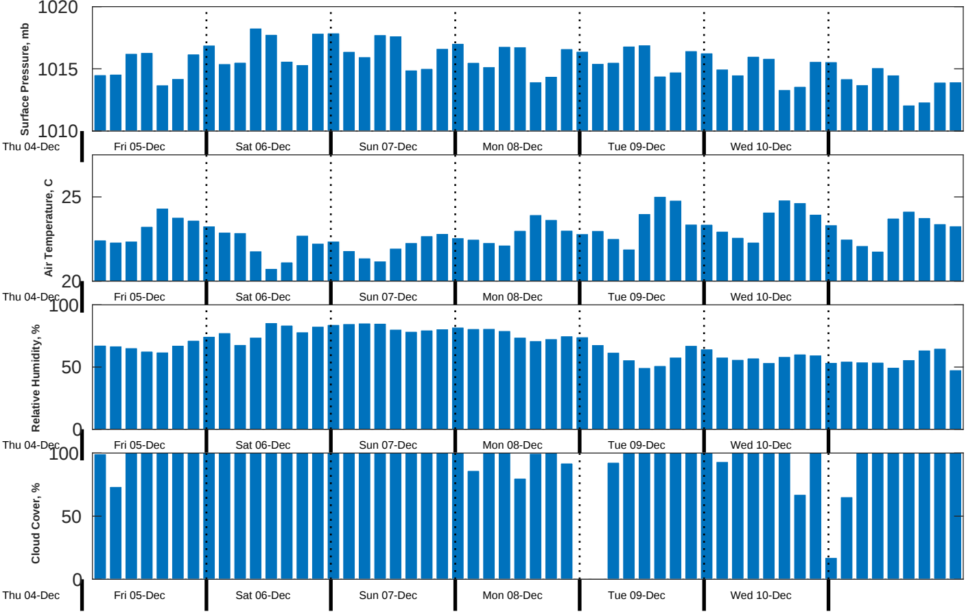
Met Forecast for CSA (ONHYM) PPL EBS - Mauritania from 05-Dec-2025 00:00:00 to 12-Dec-2025 00:00:00
