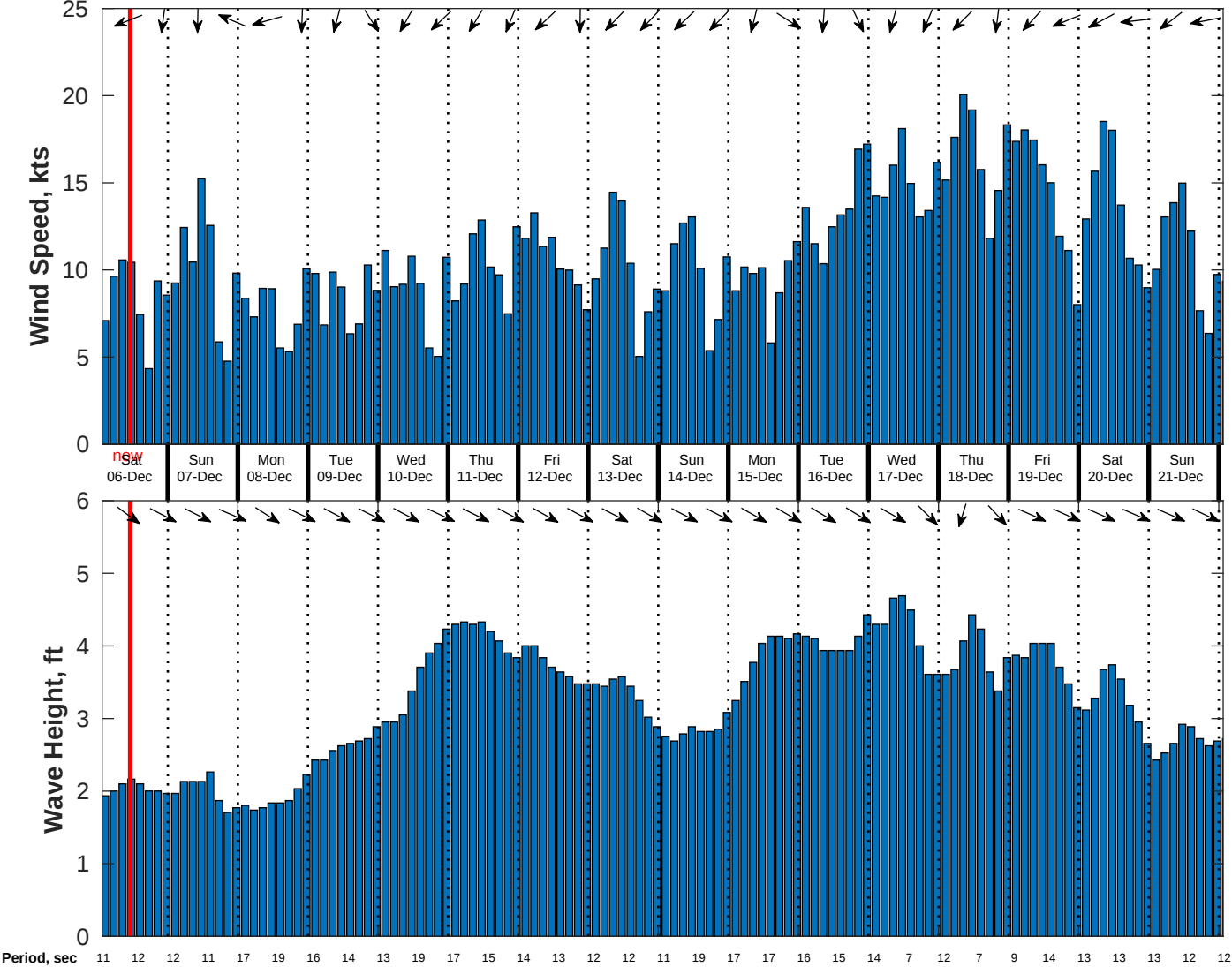
Wind & Wave Forecast for CSA (ONHYM) PPL EBS - Mauritania from 05-Dec-2025 01:00:00 to 21-Dec-2025 01:00:00
