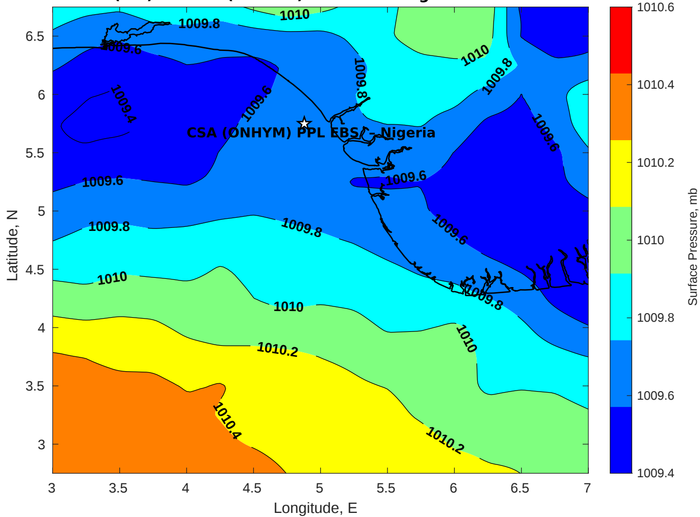
Surface Pressure (mb) for CSA (ONHYM) PPL EBS - Nigeria at 07-Dec-2025 00:00:00
