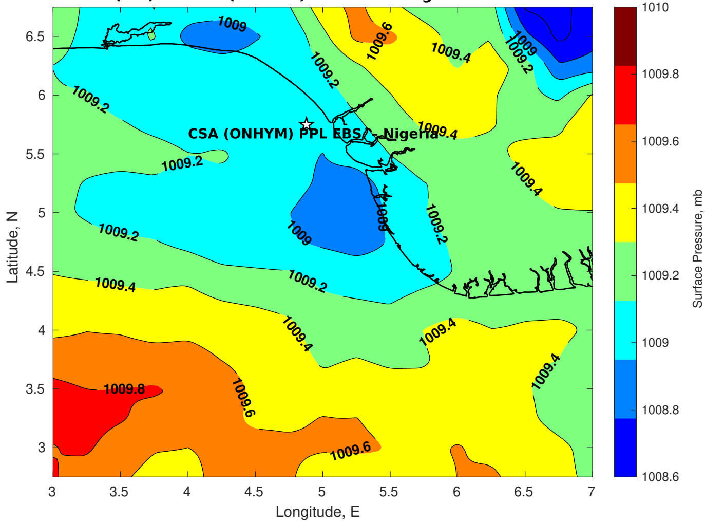
Surface Pressure (mb) for CSA (ONHYM) PPL EBS - Nigeria at 05-Dec-2025 00:00:00
