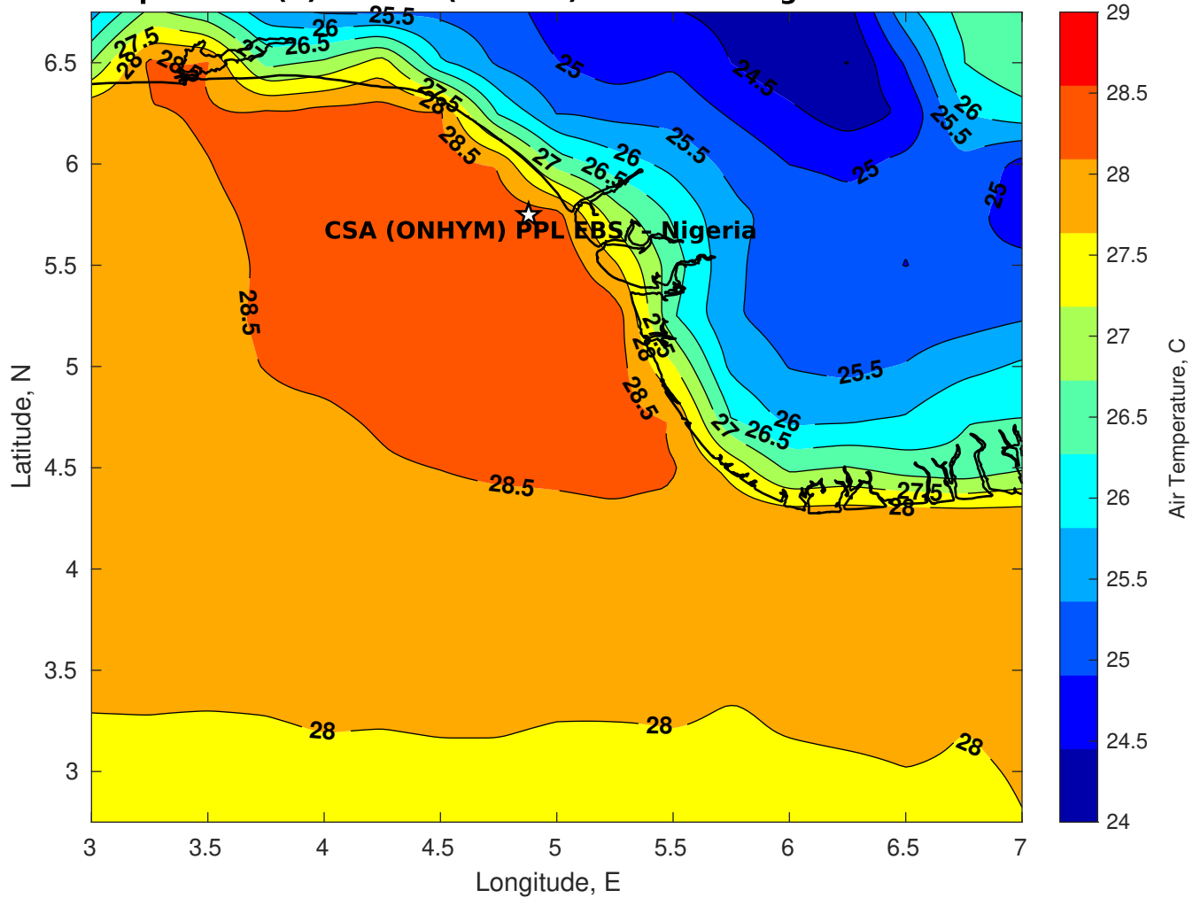
Air Temperature (C) for CSA (ONHYM) PPL EBS - Nigeria at 05-Dec-2025
