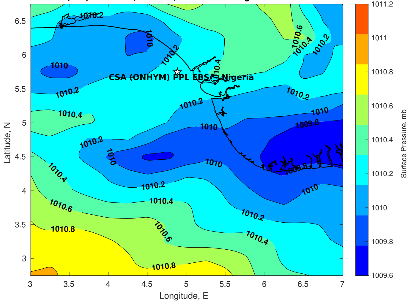
Surface Pressure (mb) for CSA (ONHYM) PPL EBS - Nigeria at 06-Dec-2025 00:00:00
