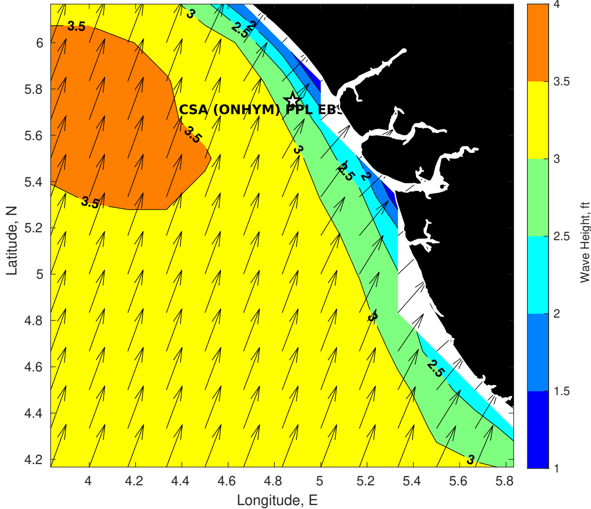
GFS Wave Height (ft) for CSA (ONHYM) PPL EBS - Nigeria at 05-Dec-2025 09:00:00
