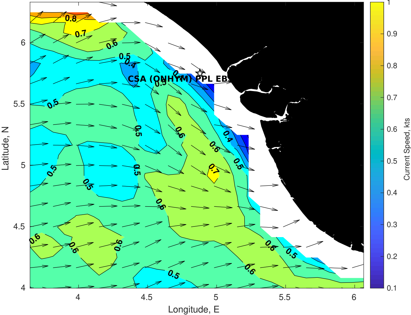
Surface Currents for CSA (ONHYM) PPL EBS - Nigeria at 04-Dec-2025 00:00:00
