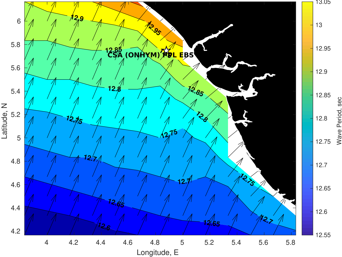
GFS Wave Period (sec) for CSA (ONHYM) PPL EBS - Nigeria at 05-Dec-2025 09:00:00
