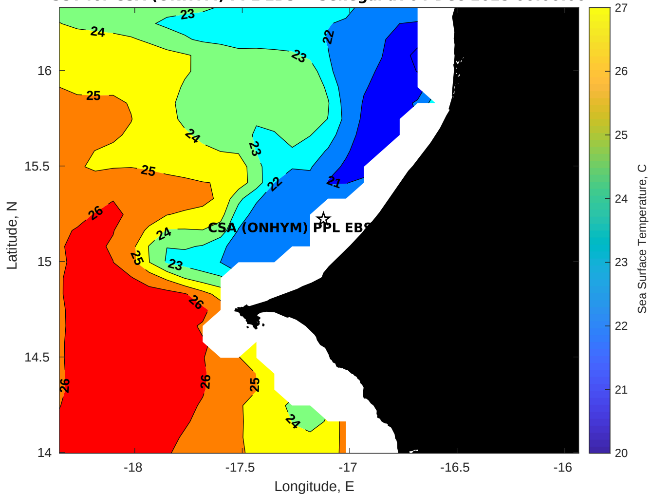
SST for CSA (ONHYM) PPL EBS - Senegal at 04-Dec-2025 00:00:00
