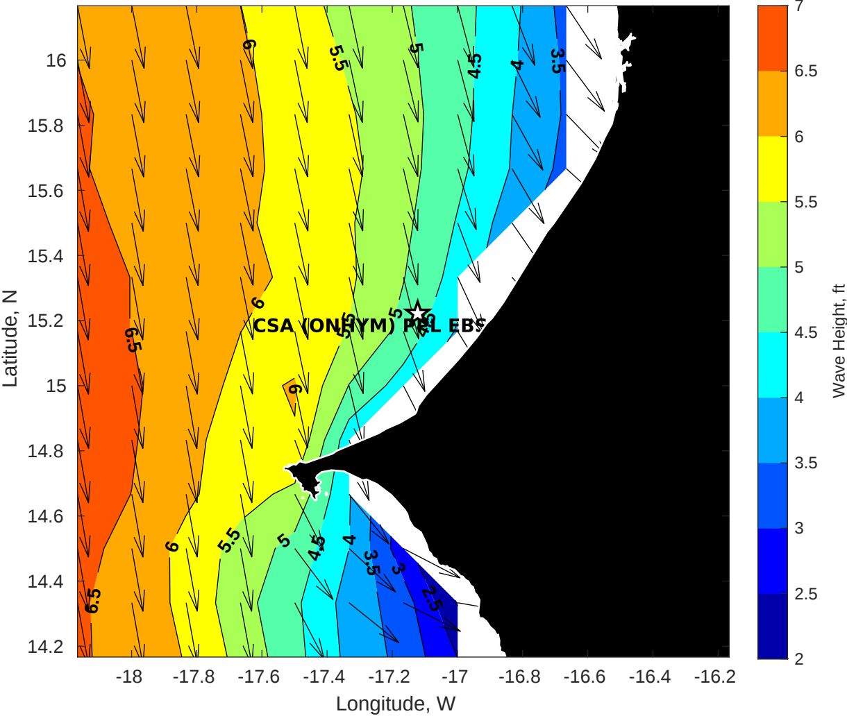
GFS Wave Height (ft) for CSA (ONHYM) PPL EBS - Senegal at 05-Dec-2025 09:00:00
