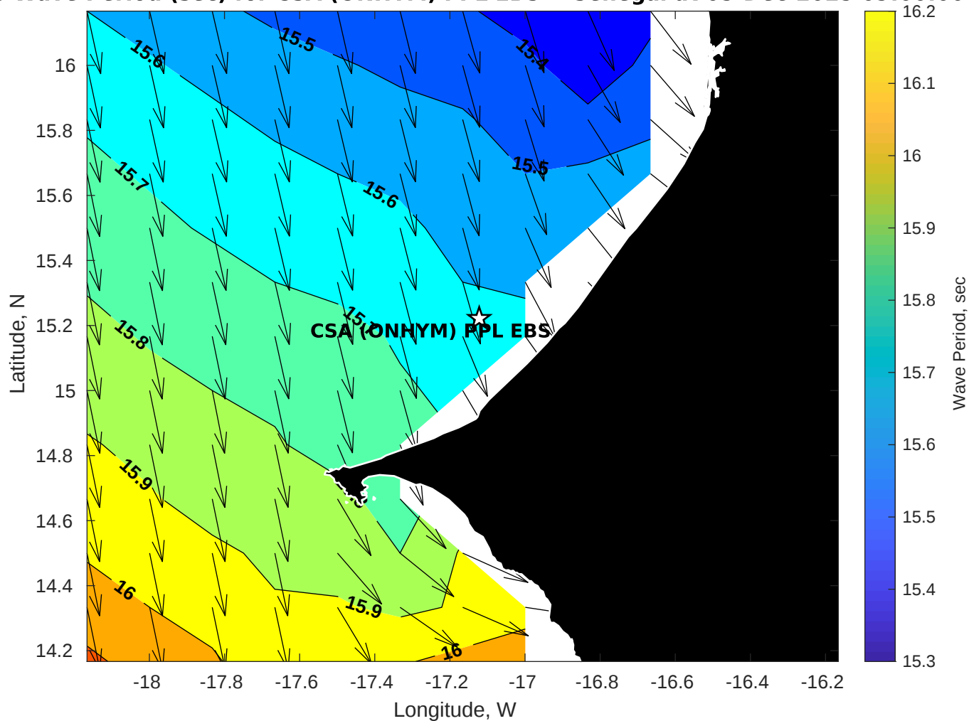
GFS Wave Period (sec) for CSA (ONHYM) PPL EBS - Senegal at 05-Dec-2025 09:00:00
