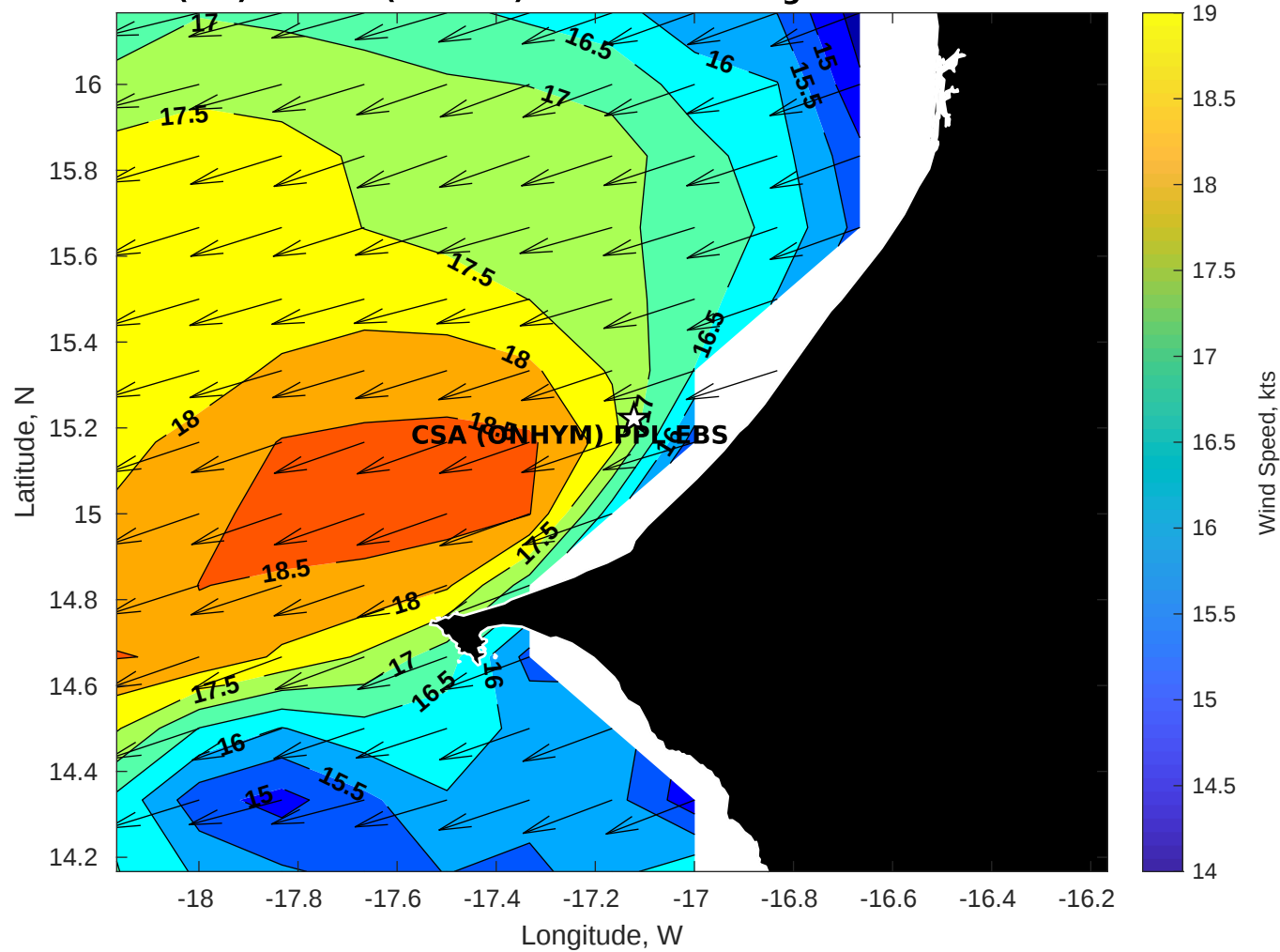
GFS Winds (kts) for CSA (ONHYM) PPL EBS - Senegal at 05-Dec-2025 09:00:00
