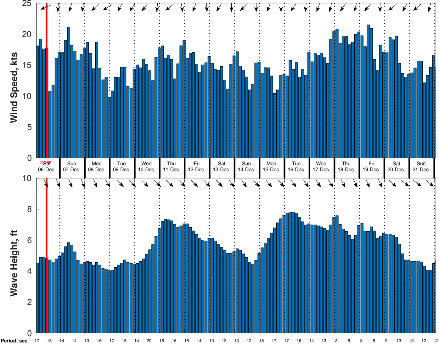
Wind & Wave Forecast for CSA (ONHYM) PPL EBS - Senegal from 05-Dec-2025 01:00:00 to 21-Dec-2025 01:00:00
