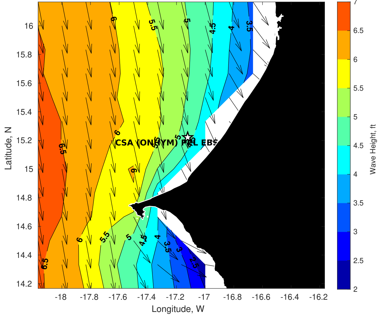
GFS Wave Height (ft) for CSA (ONHYM) PPL EBS - Senegal at 05-Dec-2025 09:00:00
