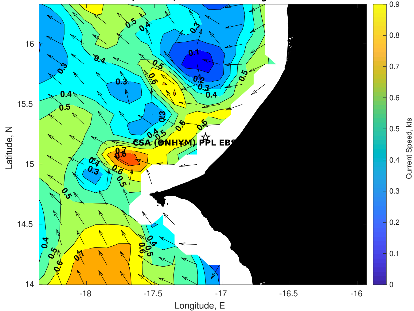
Surface Currents for CSA (ONHYM) PPL EBS - Senegal at 04-Dec-2025 00:00:00
