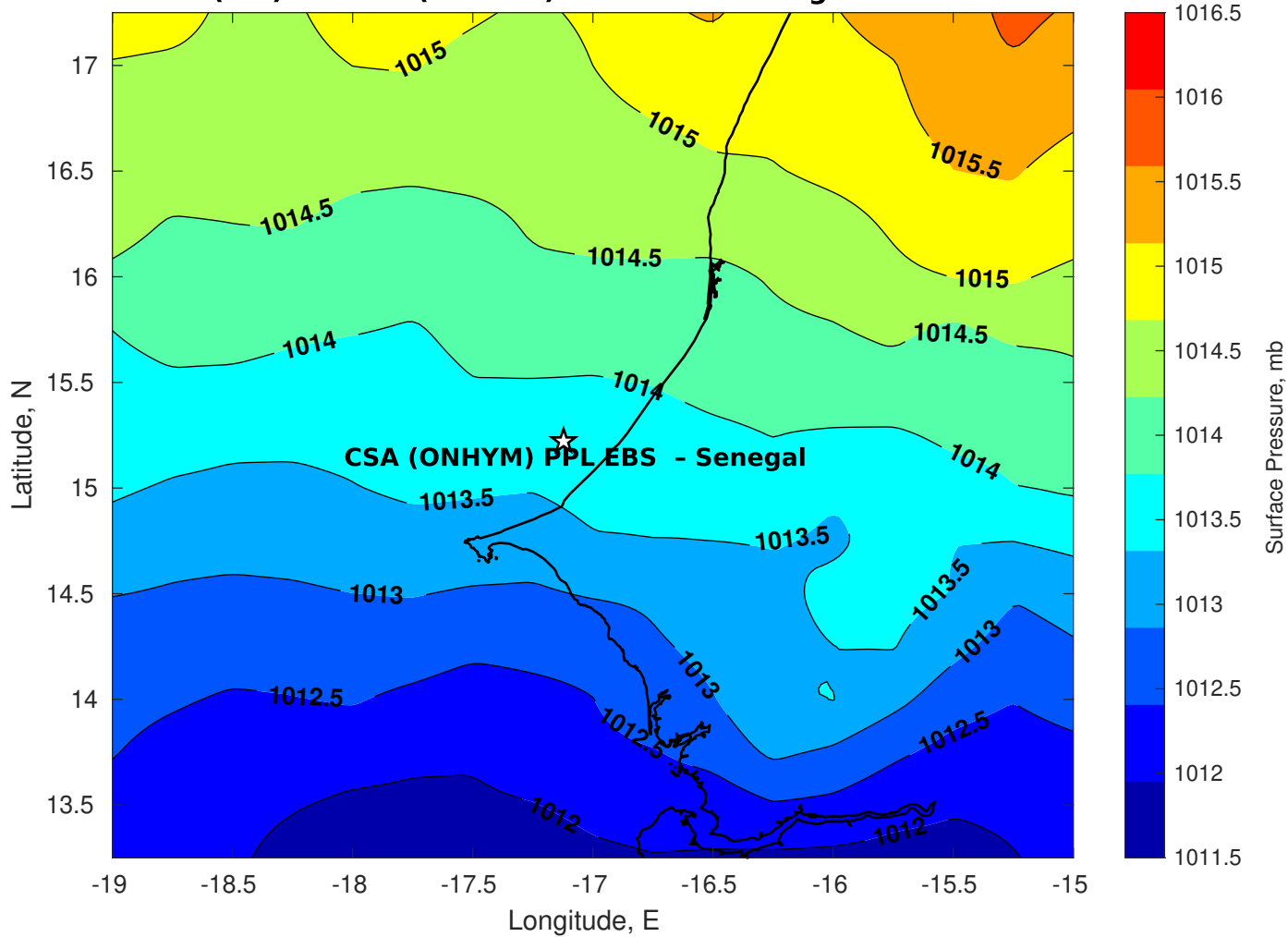
Surface Pressure (mb) for CSA (ONHYM) PPL EBS - Senegal at 05-Dec-2025 00:00:00
