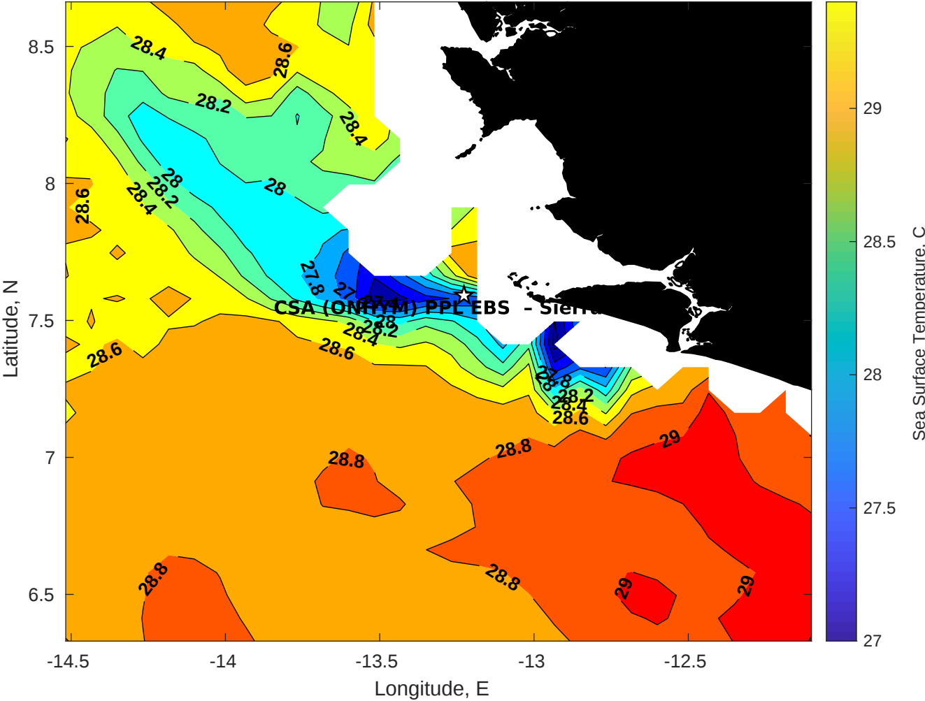
SST for CSA (ONHYM) PPL EBS - Sierra Leone at 04-Dec-2025 00:00:00
