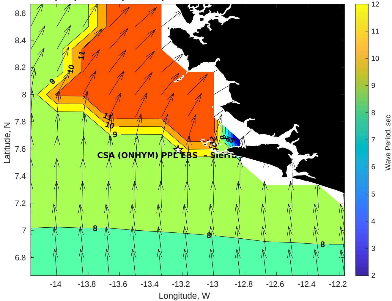
GFS Wave Period (sec) for CSA (ONHYM) PPL EBS - Sierra Leone at 05-Dec-2025 09:00:00
